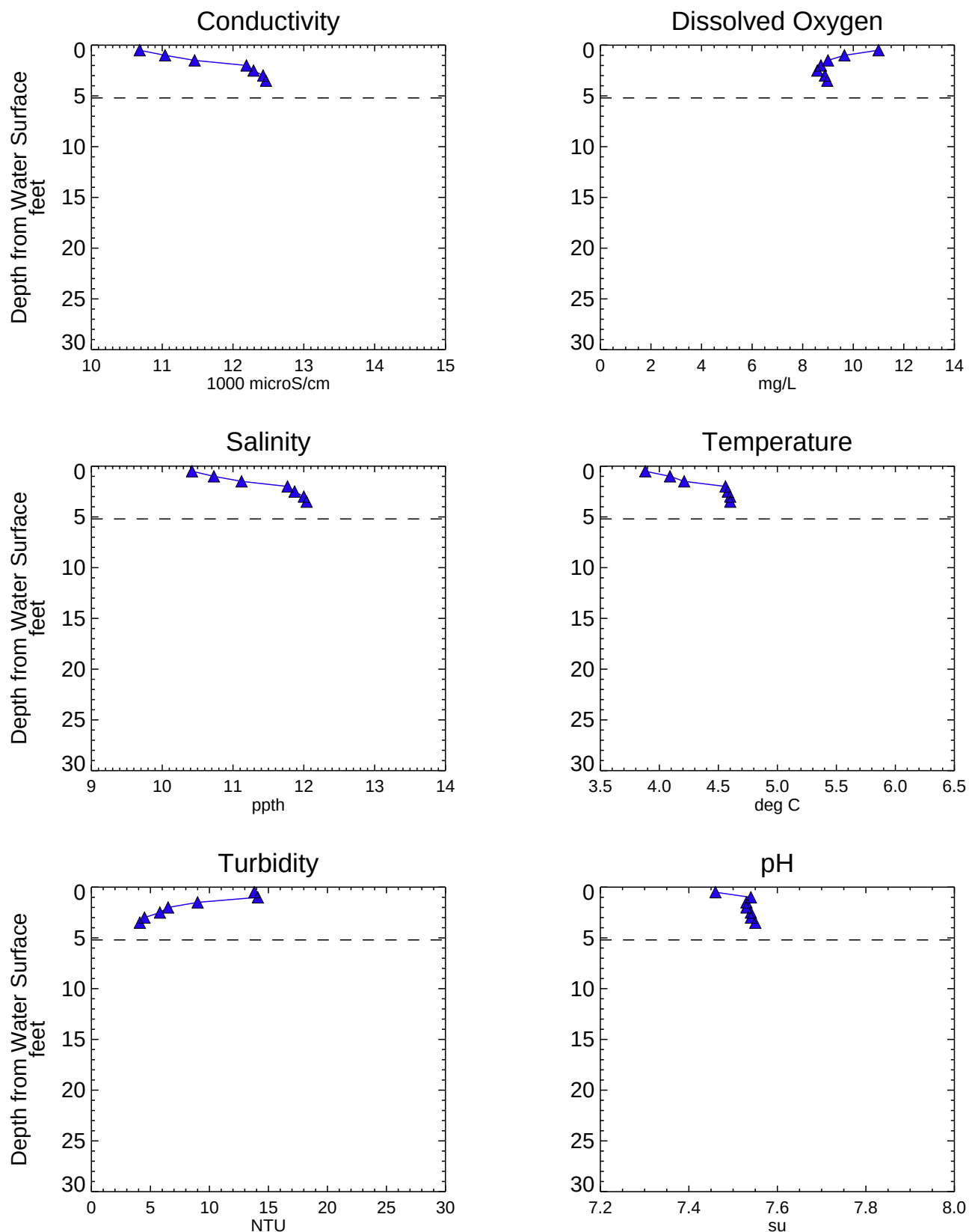
Figure A3-10 Analytical Water Quality Depth Profiles - MC008SW Phase 1 RI Data Summary Report - Submittal No. 1 Newtown Creek RI/FS
