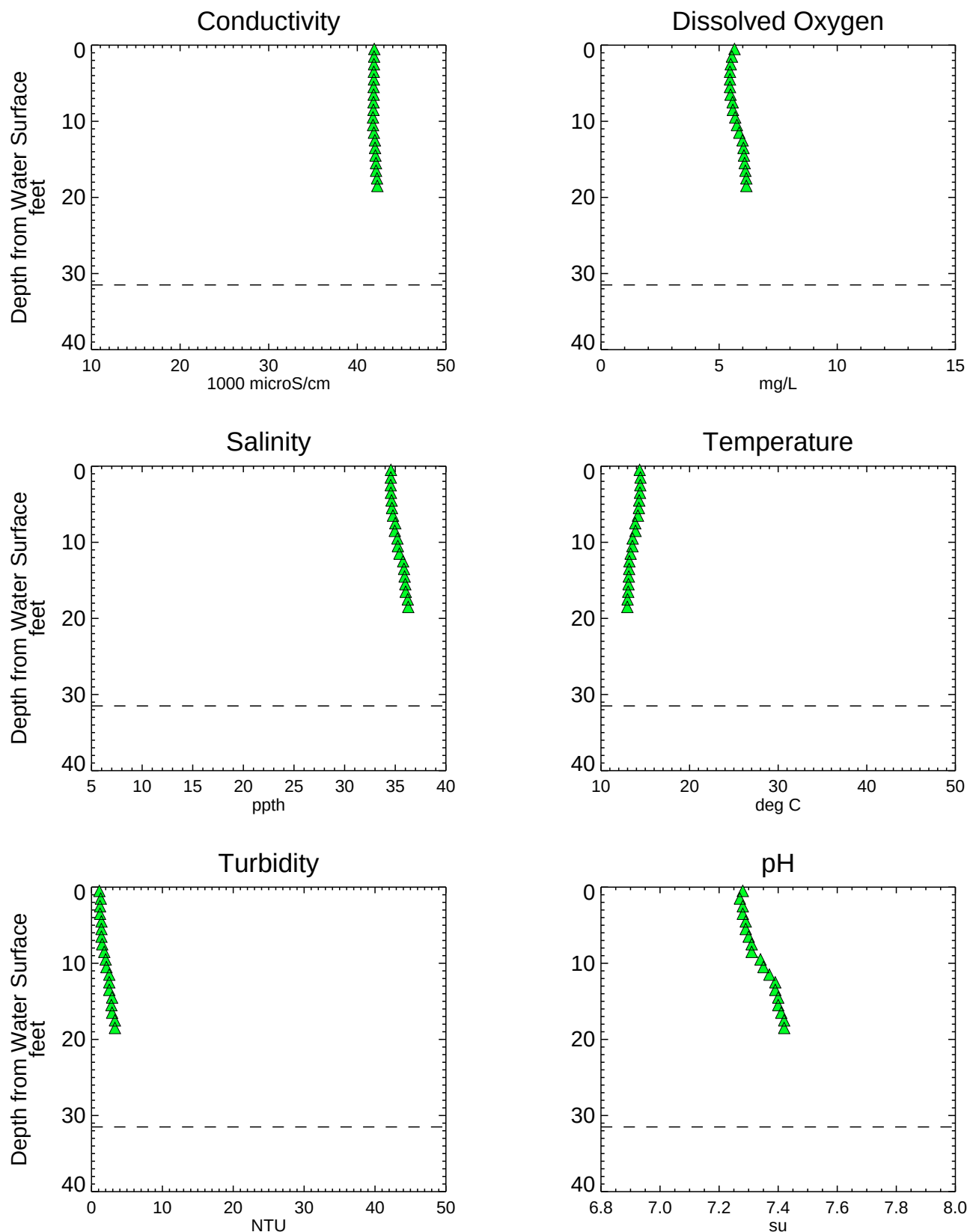
Figure A3-48 Analytical Water Quality Depth Profiles - NC020SW Phase 1 RI Data Summary Report - Submittal No. 1 Newtown Creek RI/FS
