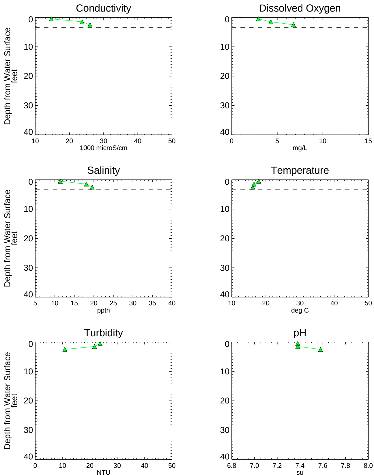
Figure A3-56 Analytical Water Quality Depth Profiles - MC008SW Phase 1 RI Data Summary Report - Submittal No. 1 Newtown Creek RI/FS
