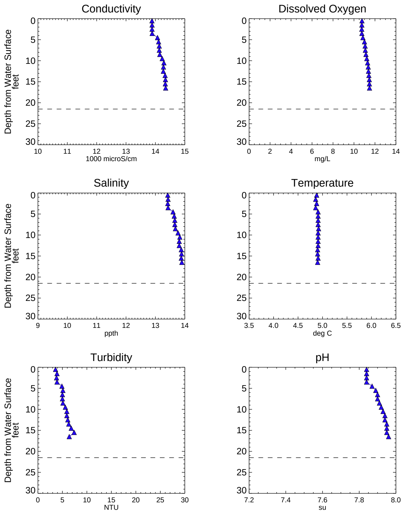
Figure A3-3 Analytical Water Quality Depth Profiles - DK001SW Phase 1 RI Data Summary Report - Submittal No. 1 Newtown Creek RI/FS
