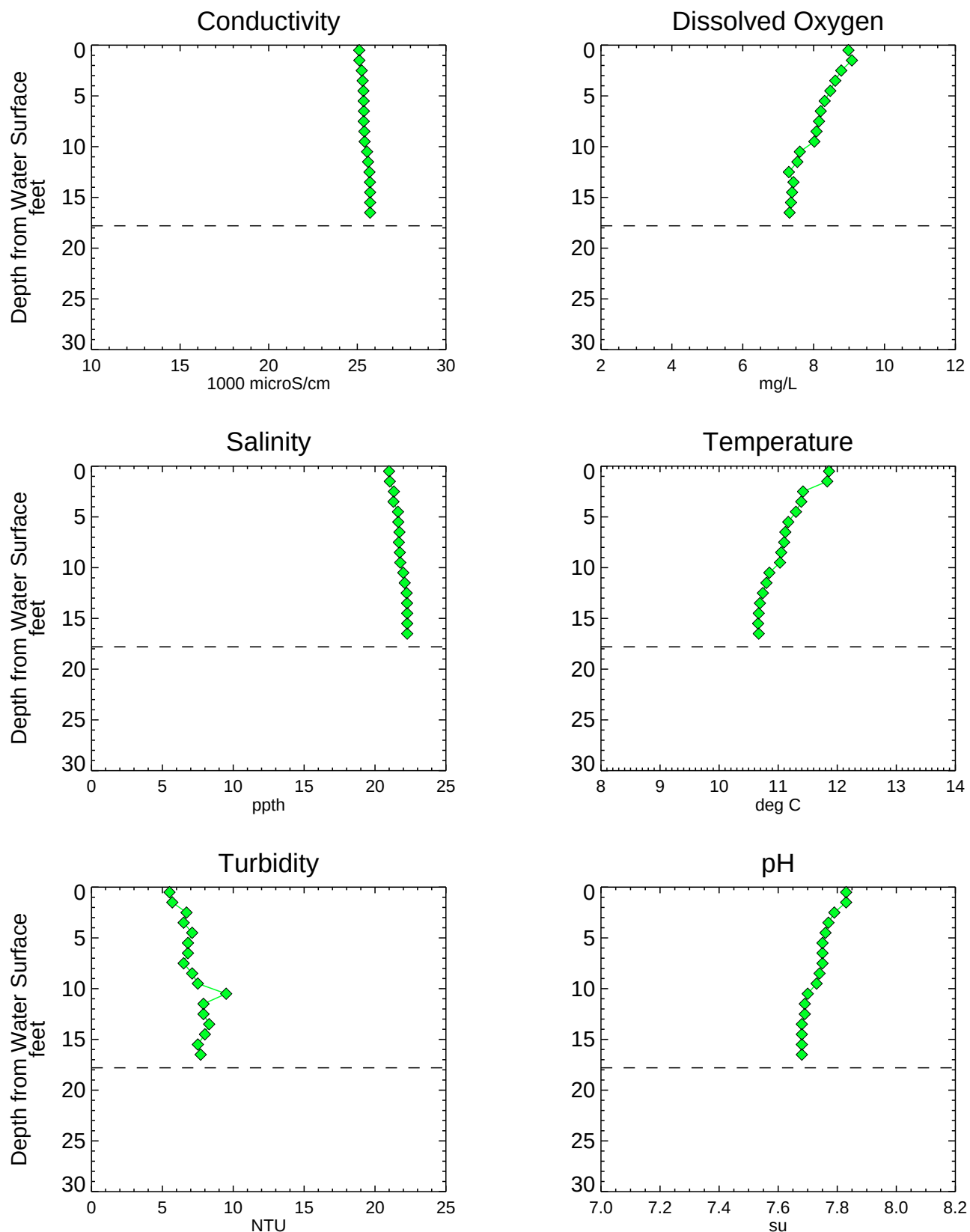
Figure A3-40 Analytical Water Quality Depth Profiles - NC070SW Phase 1 RI Data Summary Report - Submittal No. 1 Newtown Creek RI/FS
