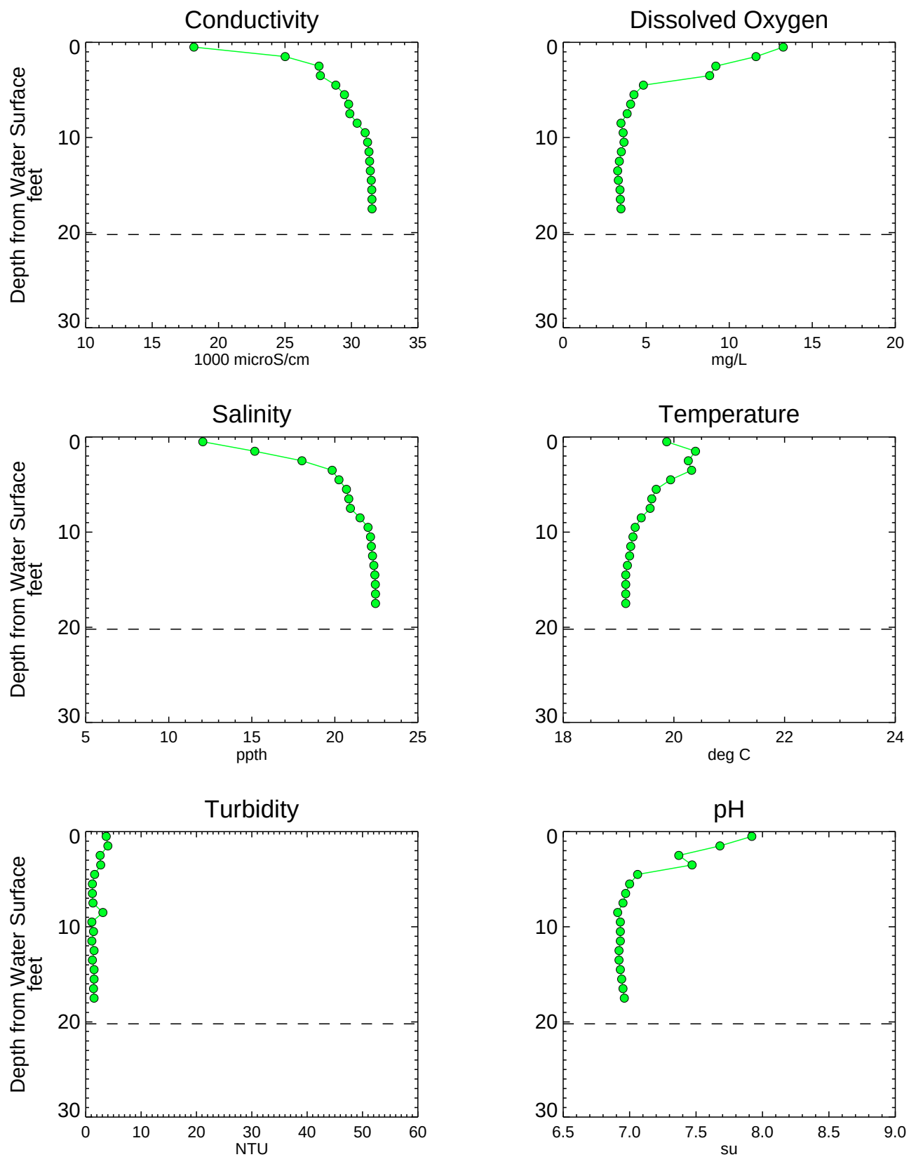
Figure A3-69 Analytical Water Quality Depth Profiles - NC068SW Phase 1 RI Data Summary Report - Submittal No. 1 Newtown Creek RI/FS
