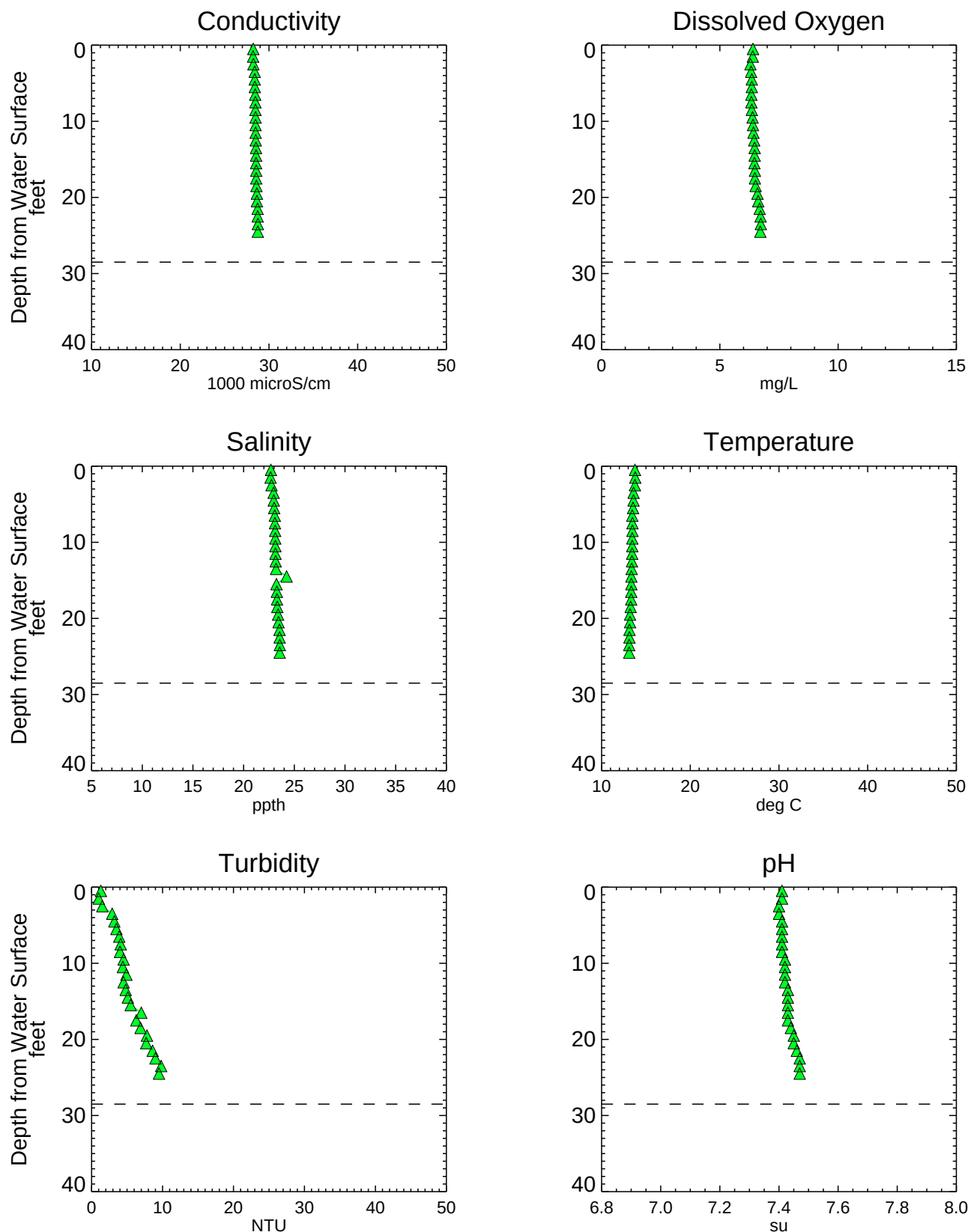
Figure A3-50 Analytical Water Quality Depth Profiles - WC001SW Phase 1 RI Data Summary Report - Submittal No. 1 Newtown Creek RI/FS
