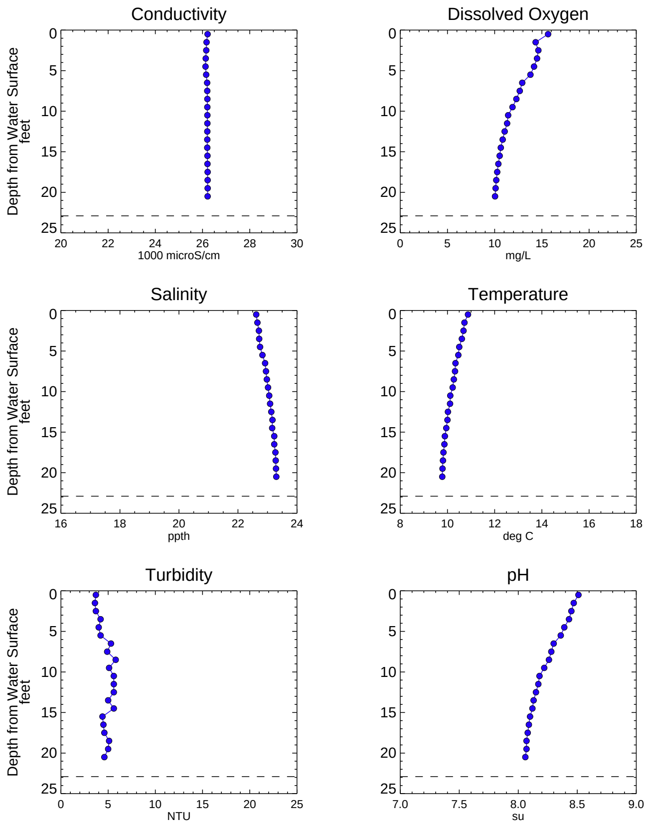
Figure A3-17 Analytical Water Quality Depth Profiles - NC020SW Phase 1 RI Data Summary Report - Submittal No. 1 Newtown Creek RI/FS
