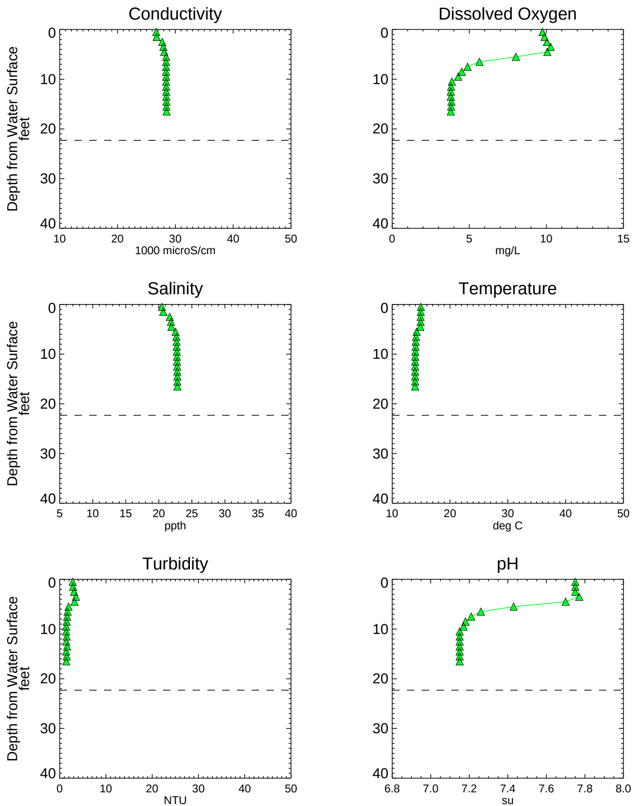
Figure A3-58 Analytical Water Quality Depth Profiles - EK006SW Phase 1 RI Data Summary Report - Submittal No. 1 Newtown Creek RI/FS
