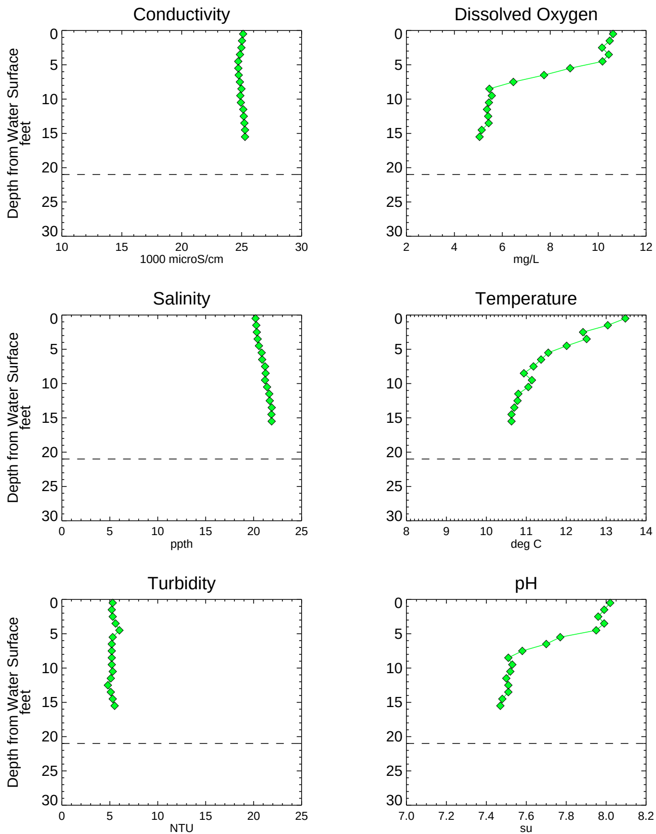
Figure A3-43 Analytical Water Quality Depth Profiles - EK006SW Phase 1 RI Data Summary Report - Submittal No. 1 Newtown Creek RI/FS
