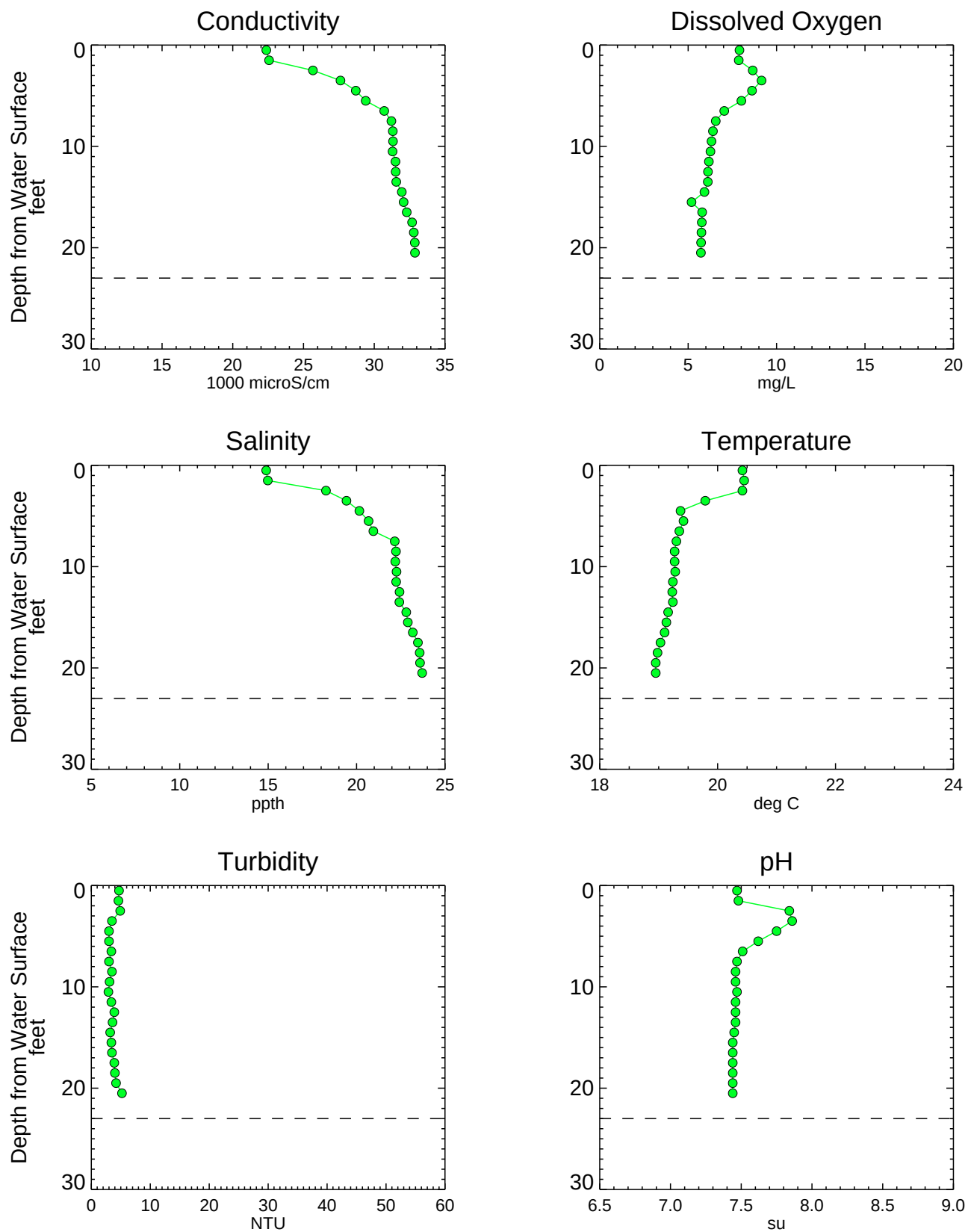
Figure A3-63 Analytical Water Quality Depth Profiles - NC020SW Phase 1 RI Data Summary Report - Submittal No. 1 Newtown Creek RI/FS
