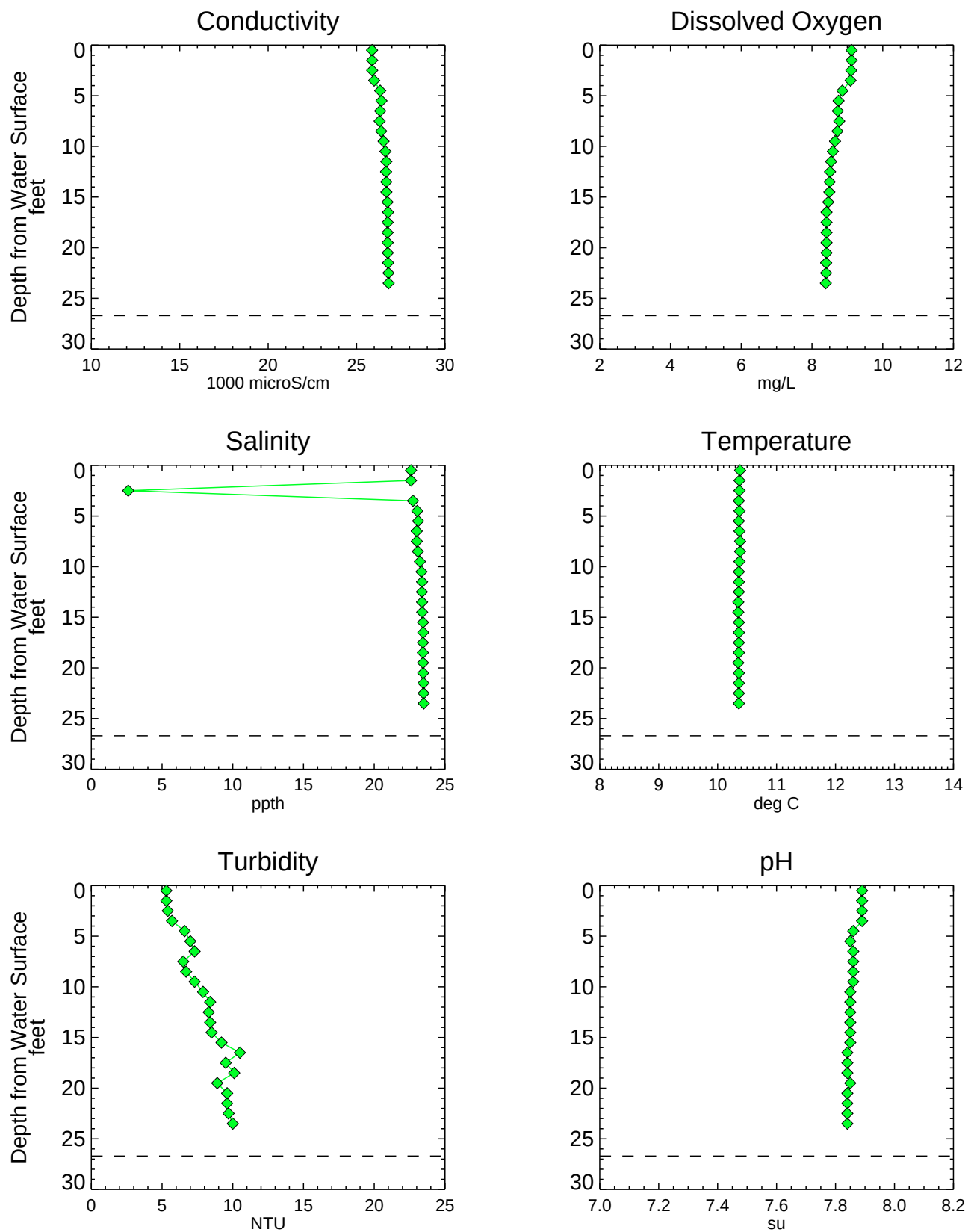
Figure A3-38 Analytical Water Quality Depth Profiles - NC046SW Phase 1 RI Data Summary Report - Submittal No. 1 Newtown Creek RI/FS
