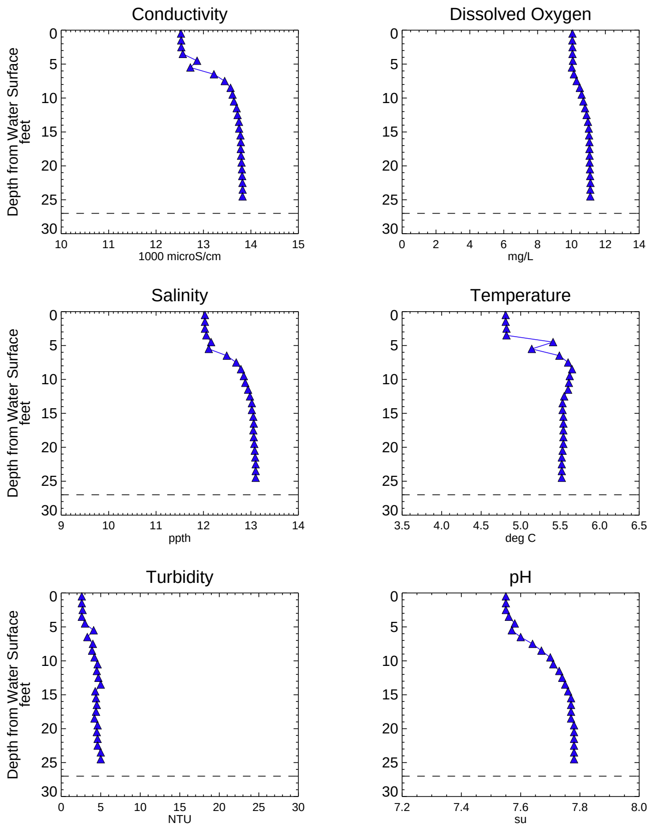
Figure A3-5 Analytical Water Quality Depth Profiles - NC034SW Phase 1 RI Data Summary Report - Submittal No. 1 Newtown Creek RI/FS
