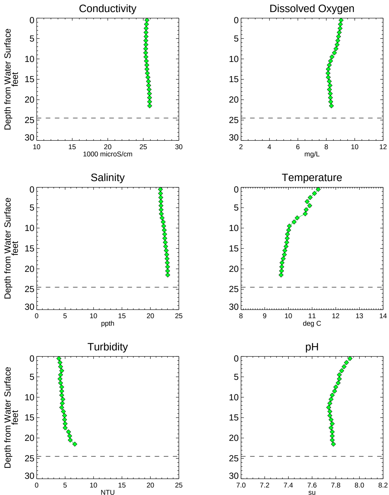
Figure A3-34 Analytical Water Quality Depth Profiles - WC001SW Phase 1 RI Data Summary Report - Submittal No. 1 Newtown Creek RI/FS
