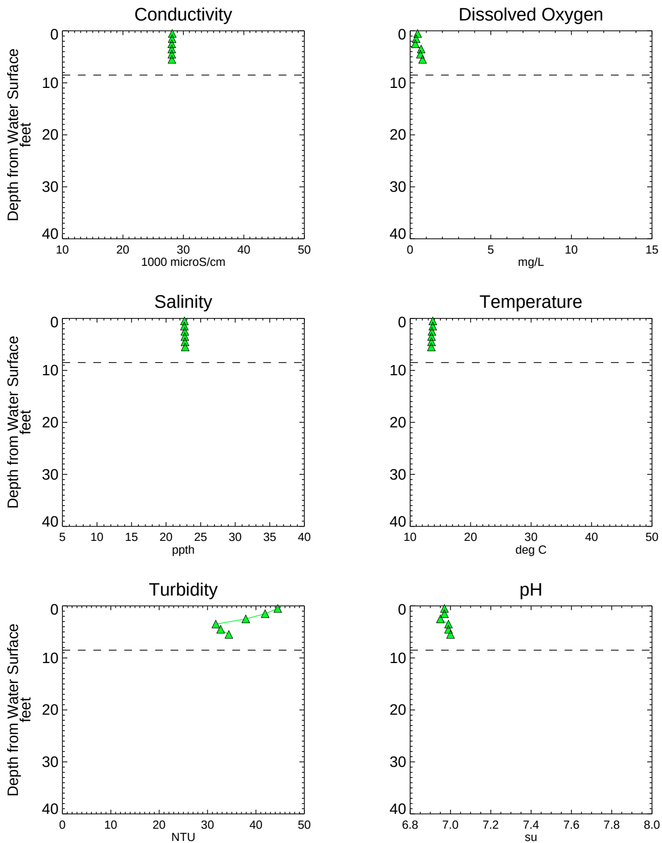
Figure A3-59 Analytical Water Quality Depth Profiles - EB010SW Phase 1 RI Data Summary Report - Submittal No. 1 Newtown Creek RI/FS
