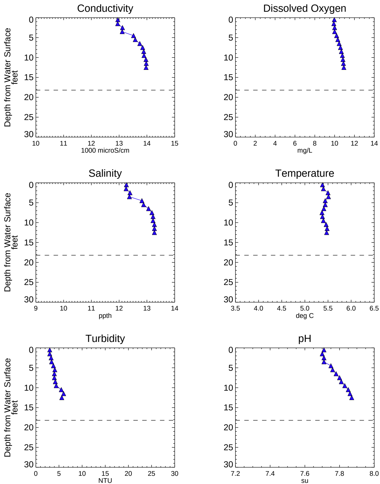
Figure A3-1 Analytical Water Quality Depth Profiles - NC007SW Phase 1 RI Data Summary Report - Submittal No. 1 Newtown Creek RI/FS
