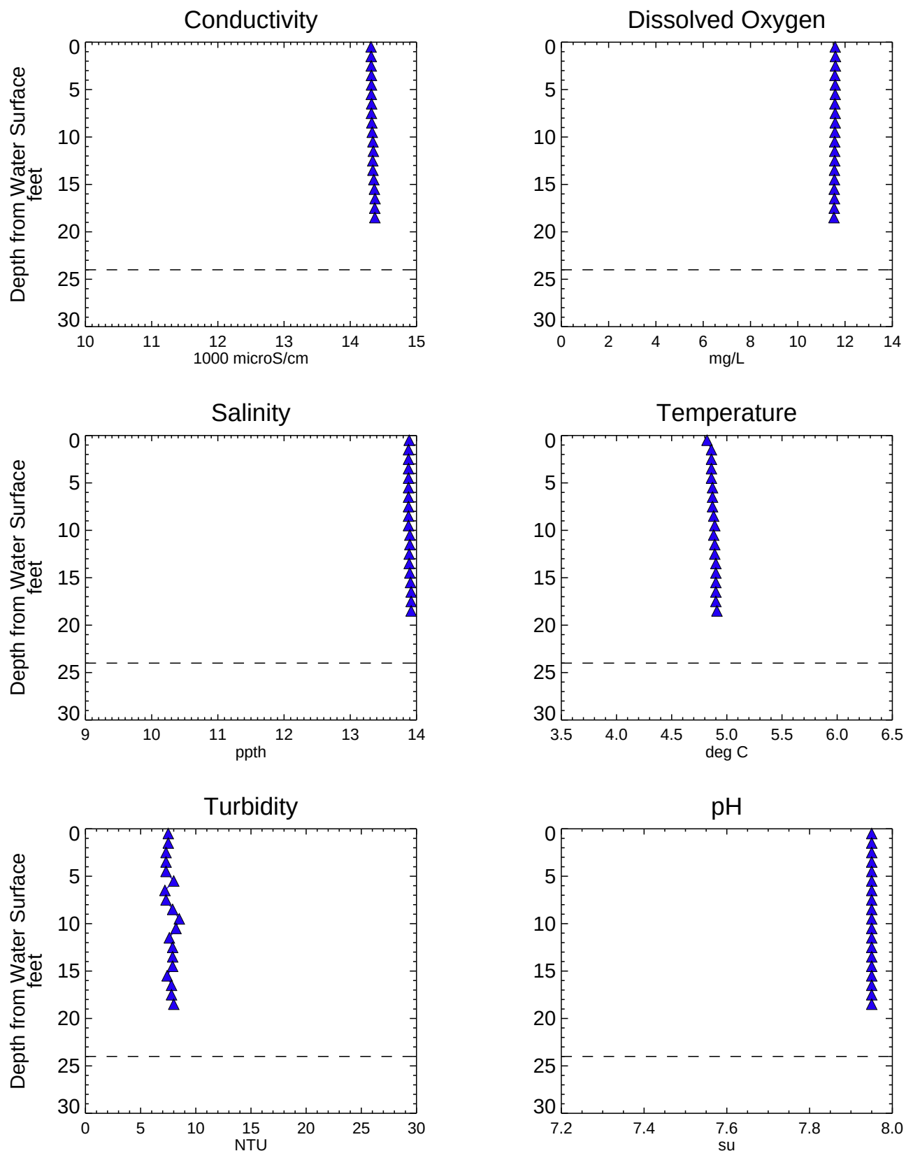
Figure A3-2 Analytical Water Quality Depth Profiles - NC020SW Phase 1 RI Data Summary Report - Submittal No. 1 Newtown Creek RI/FS
