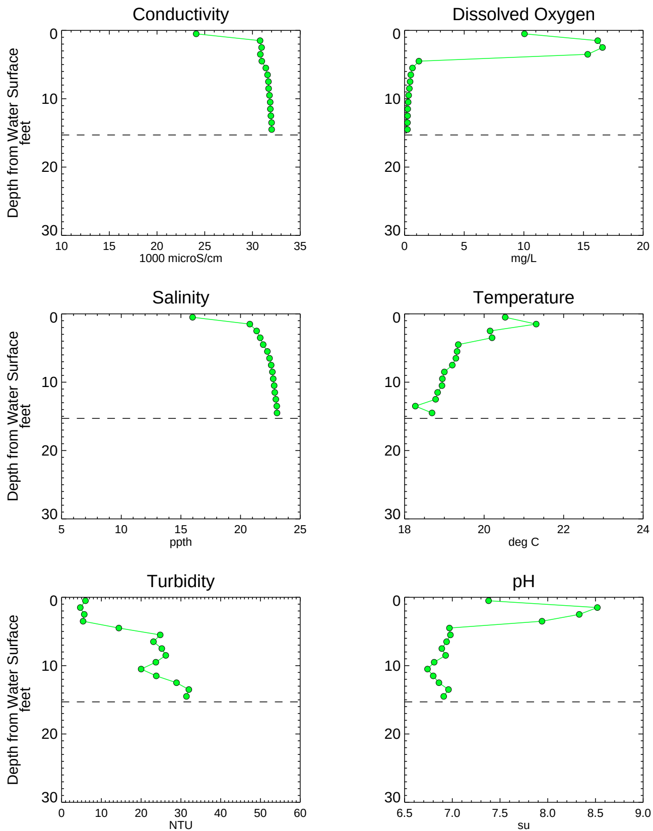
Figure A3-67 Analytical Water Quality Depth Profiles - DK011SW Phase 1 RI Data Summary Report - Submittal No. 1 Newtown Creek RI/FS
