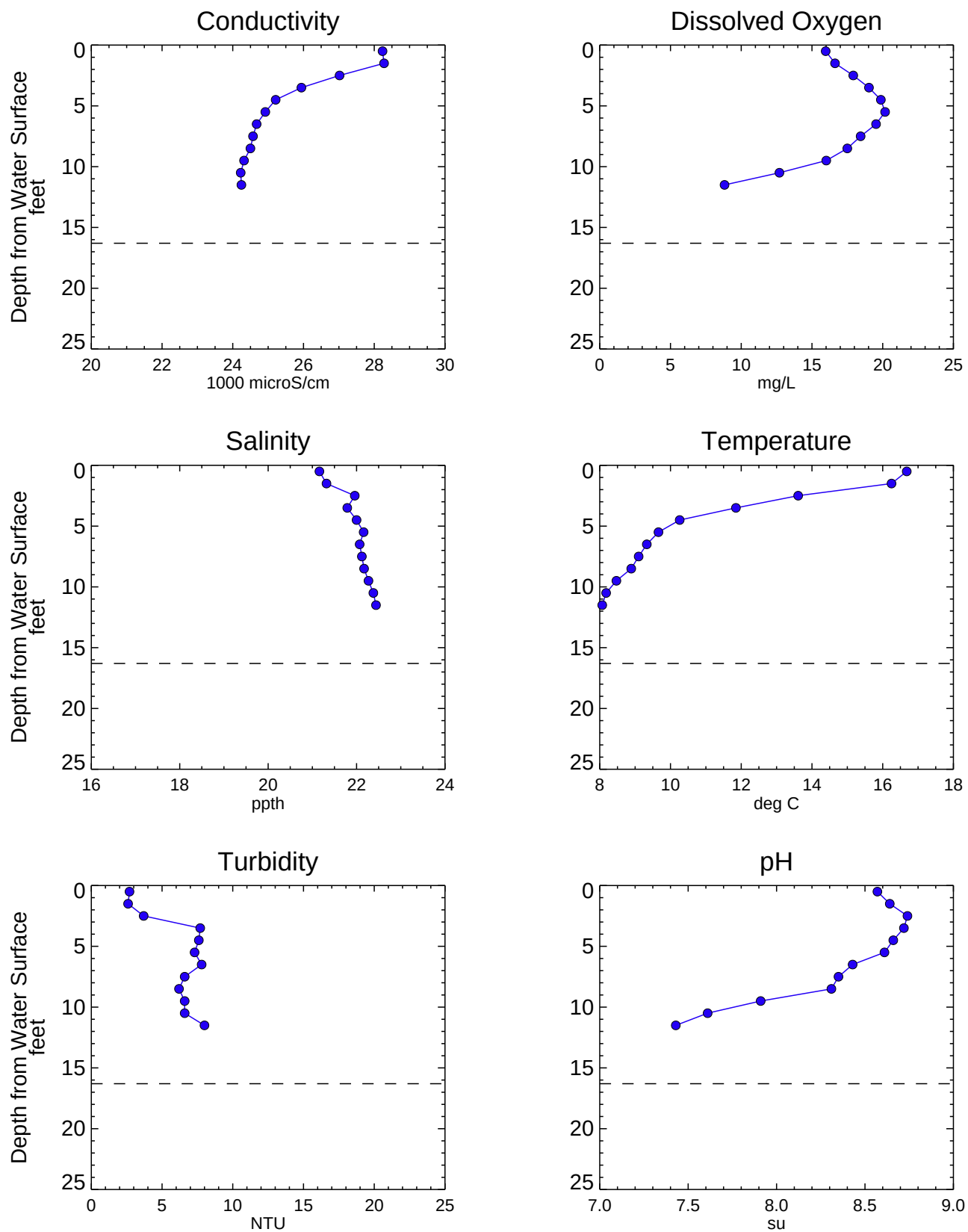
Figure A3-21 Analytical Water Quality Depth Profiles - DK011SW Phase 1 RI Data Summary Report - Submittal No. 1 Newtown Creek RI/FS
