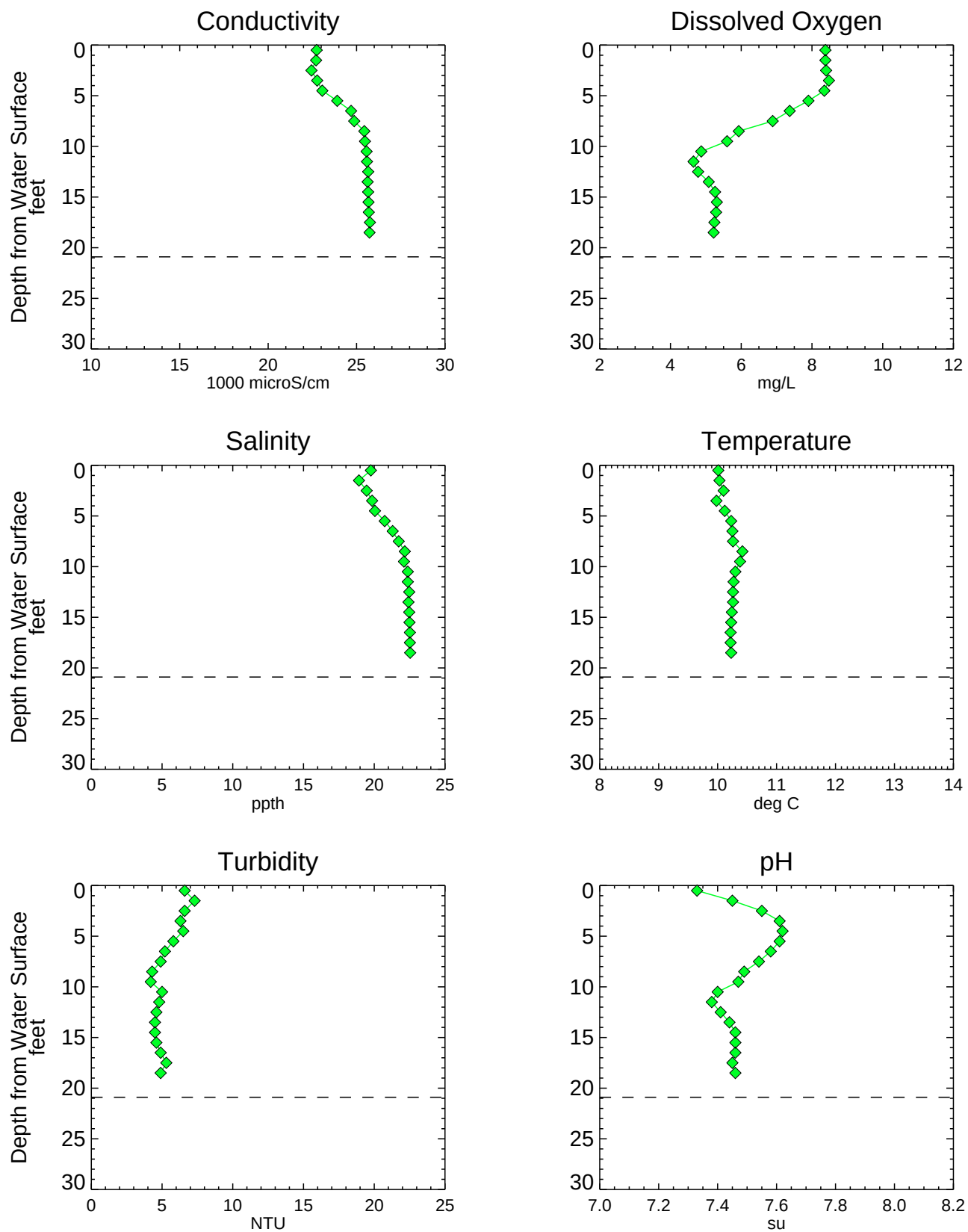
Figure A3-42 Analytical Water Quality Depth Profiles - NC079SW Phase 1 RI Data Summary Report - Submittal No. 1 Newtown Creek RI/FS
