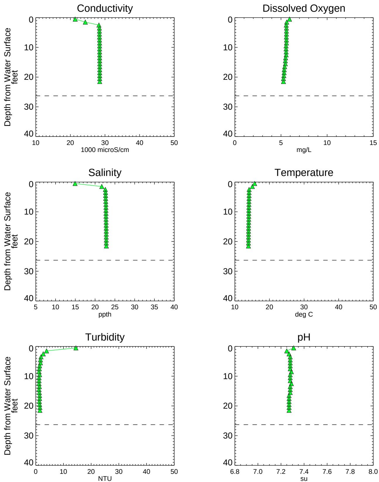
Figure A3-57 Analytical Water Quality Depth Profiles - NC079SW Phase 1 RI Data Summary Report - Submittal No. 1 Newtown Creek RI/FS
