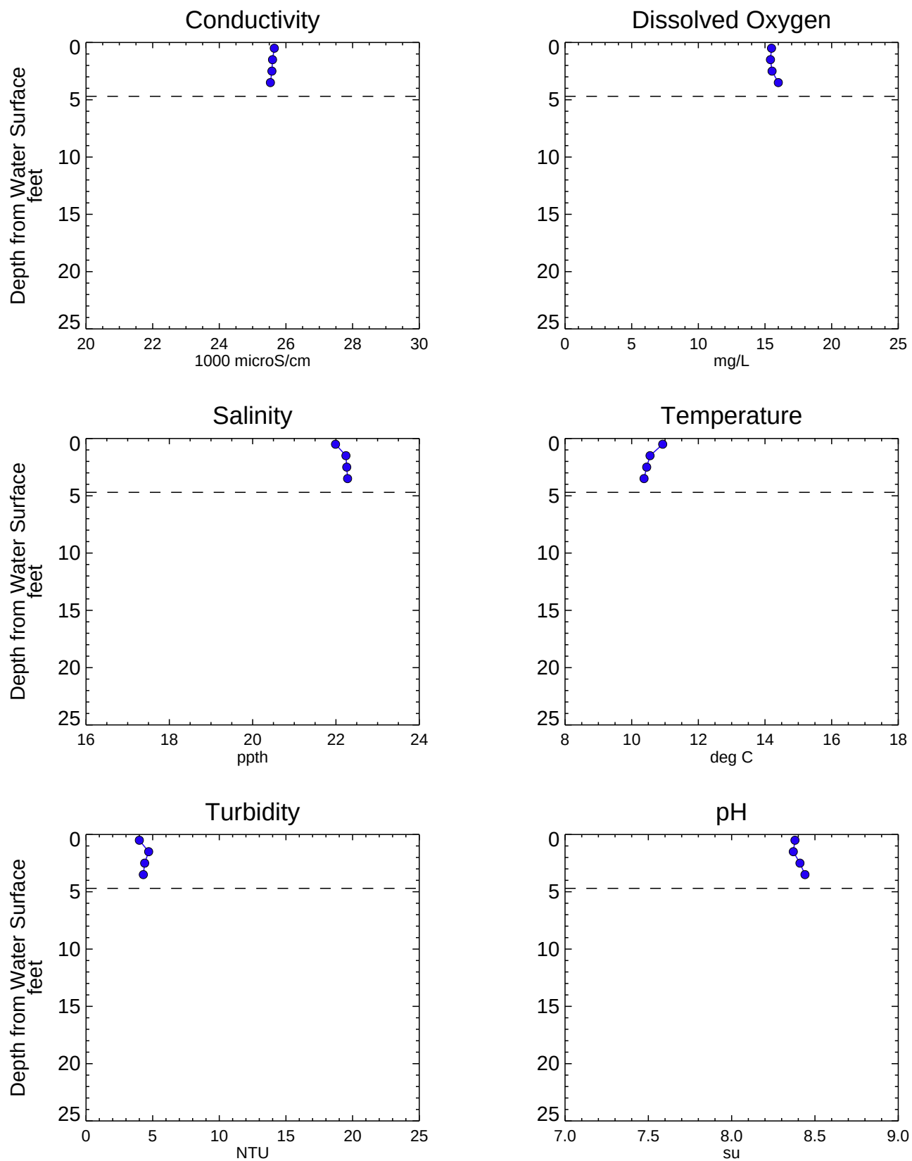
Figure A3-25 Analytical Water Quality Depth Profiles - MC008SW Phase 1 RI Data Summary Report - Submittal No. 1 Newtown Creek RI/FS
