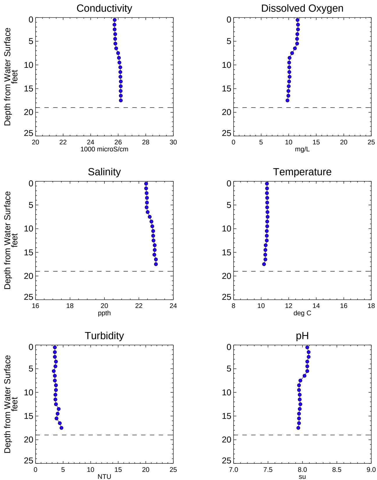
Figure A3-24 Analytical Water Quality Depth Profiles - NC070SW Phase 1 RI Data Summary Report - Submittal No. 1 Newtown Creek RI/FS
