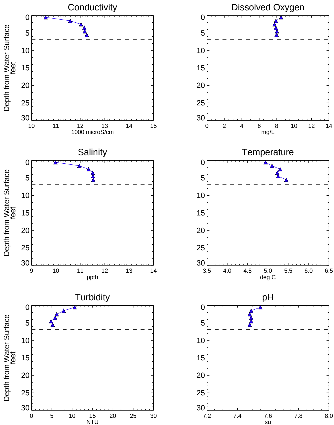
Figure A3-15 Analytical Water Quality Depth Profiles - EK022SW Phase 1 RI Data Summary Report - Submittal No. 1 Newtown Creek RI/FS
