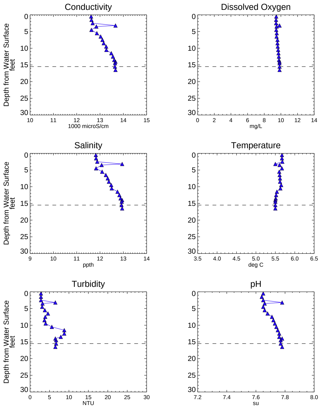
Figure A3-8 Analytical Water Quality Depth Profiles - NC068SW Phase 1 RI Data Summary Report - Submittal No. 1 Newtown Creek RI/FS
