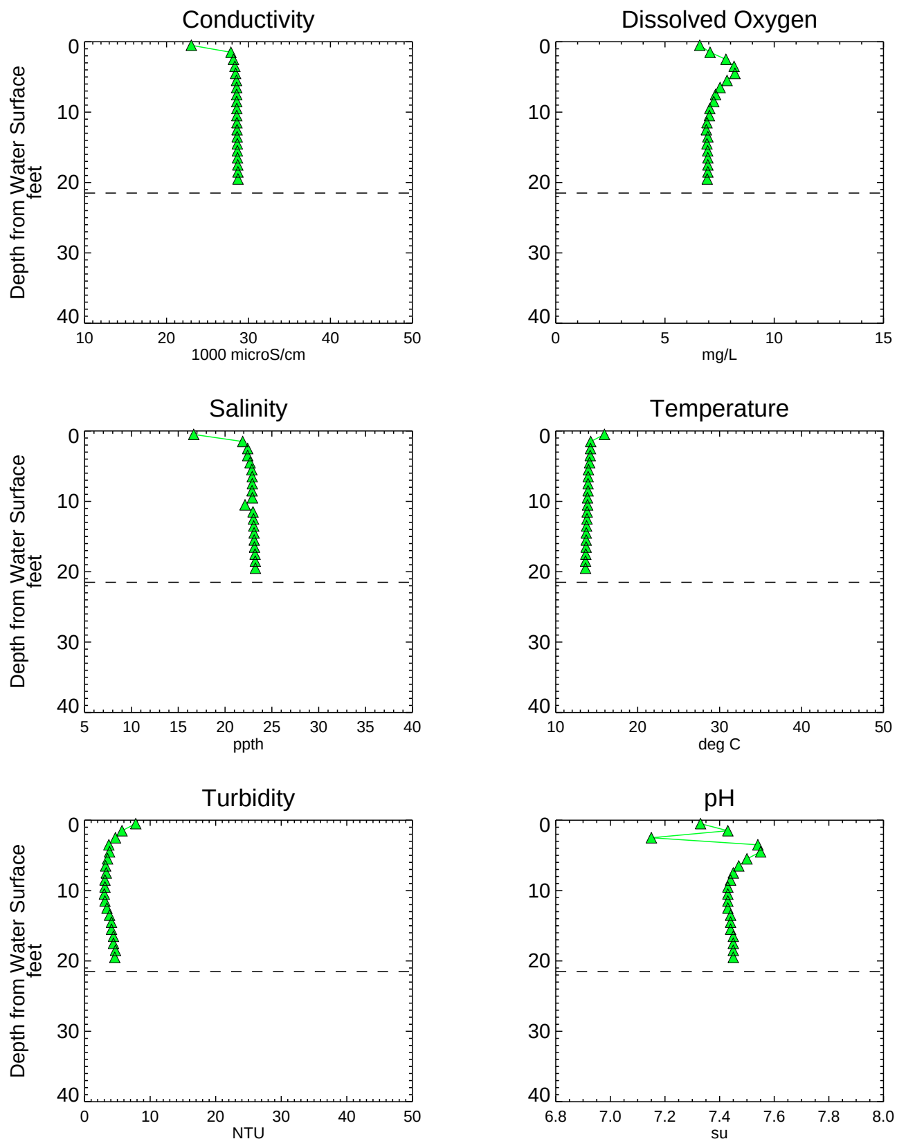
Figure A3-49 Analytical Water Quality Depth Profiles - DK001SW Phase 1 RI Data Summary Report - Submittal No. 1 Newtown Creek RI/FS
