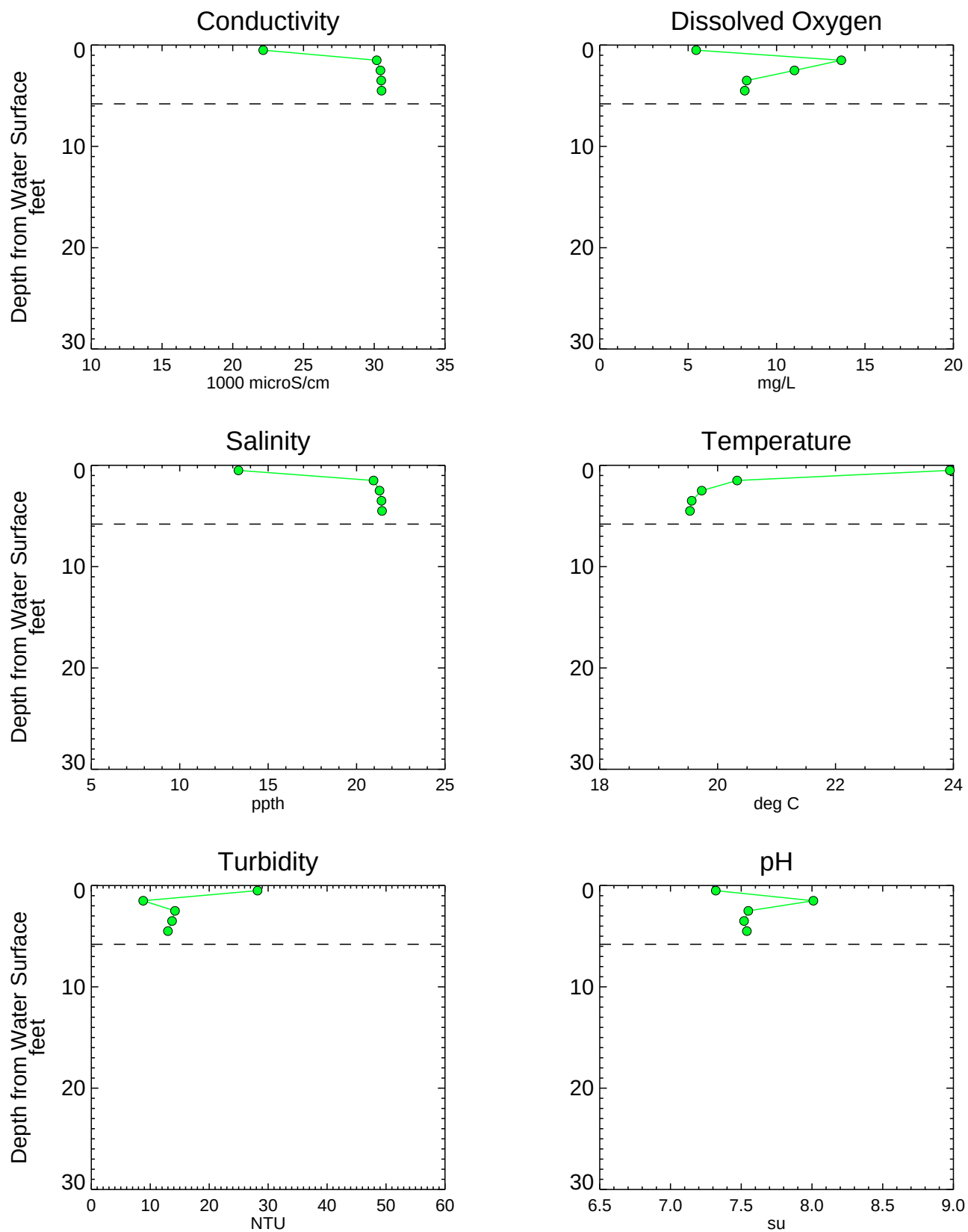
Figure A3-71 Analytical Water Quality Depth Profiles - MC008SW Phase 1 RI Data Summary Report - Submittal No. 1 Newtown Creek RI/FS
