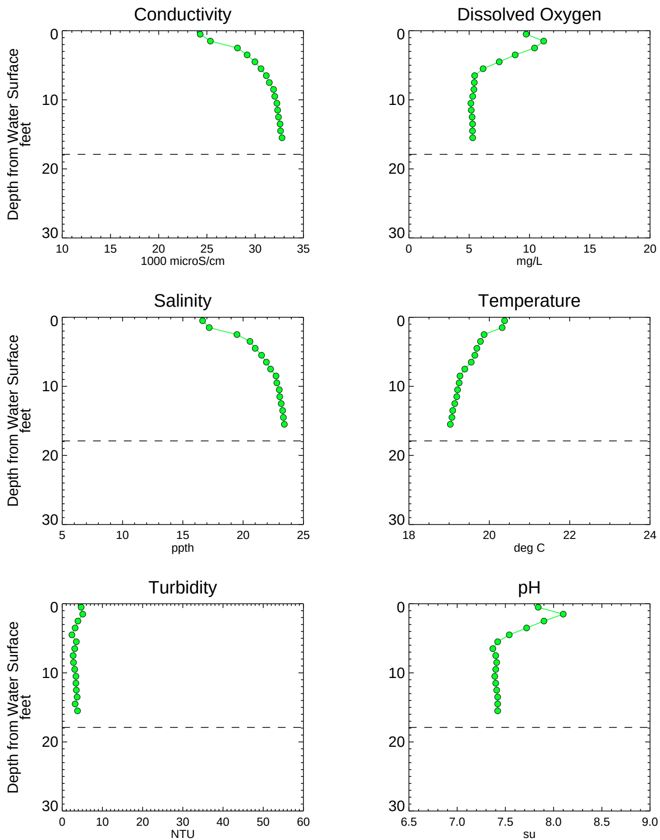
Figure A3-64 Analytical Water Quality Depth Profiles - DK001SW Phase 1 RI Data Summary Report - Submittal No. 1 Newtown Creek RI/FS
