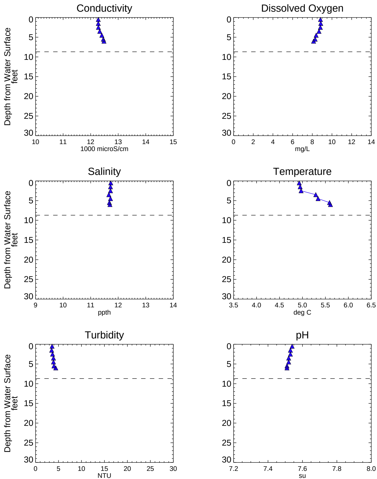
Figure A3-14 Analytical Water Quality Depth Profiles - EK014SW Phase 1 RI Data Summary Report - Submittal No. 1 Newtown Creek RI/FS
