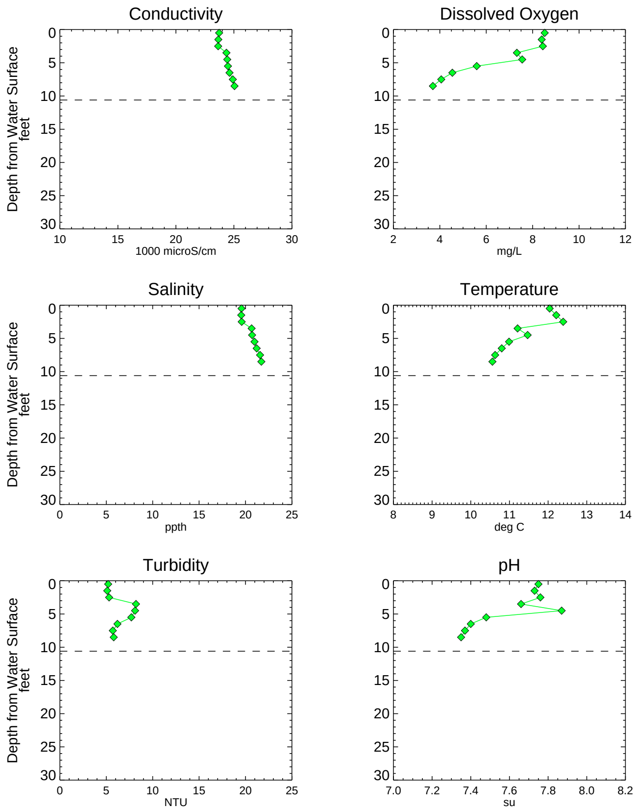
Figure A3-45 Analytical Water Quality Depth Profiles - EK014SW Phase 1 RI Data Summary Report - Submittal No. 1 Newtown Creek RI/FS
