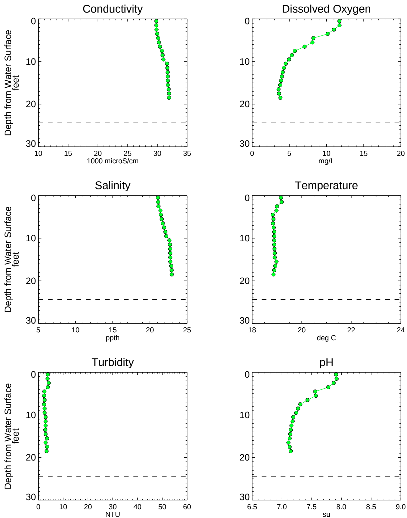
Figure A3-70 Analytical Water Quality Depth Profiles - NC070SW Phase 1 RI Data Summary Report - Submittal No. 1 Newtown Creek RI/FS
