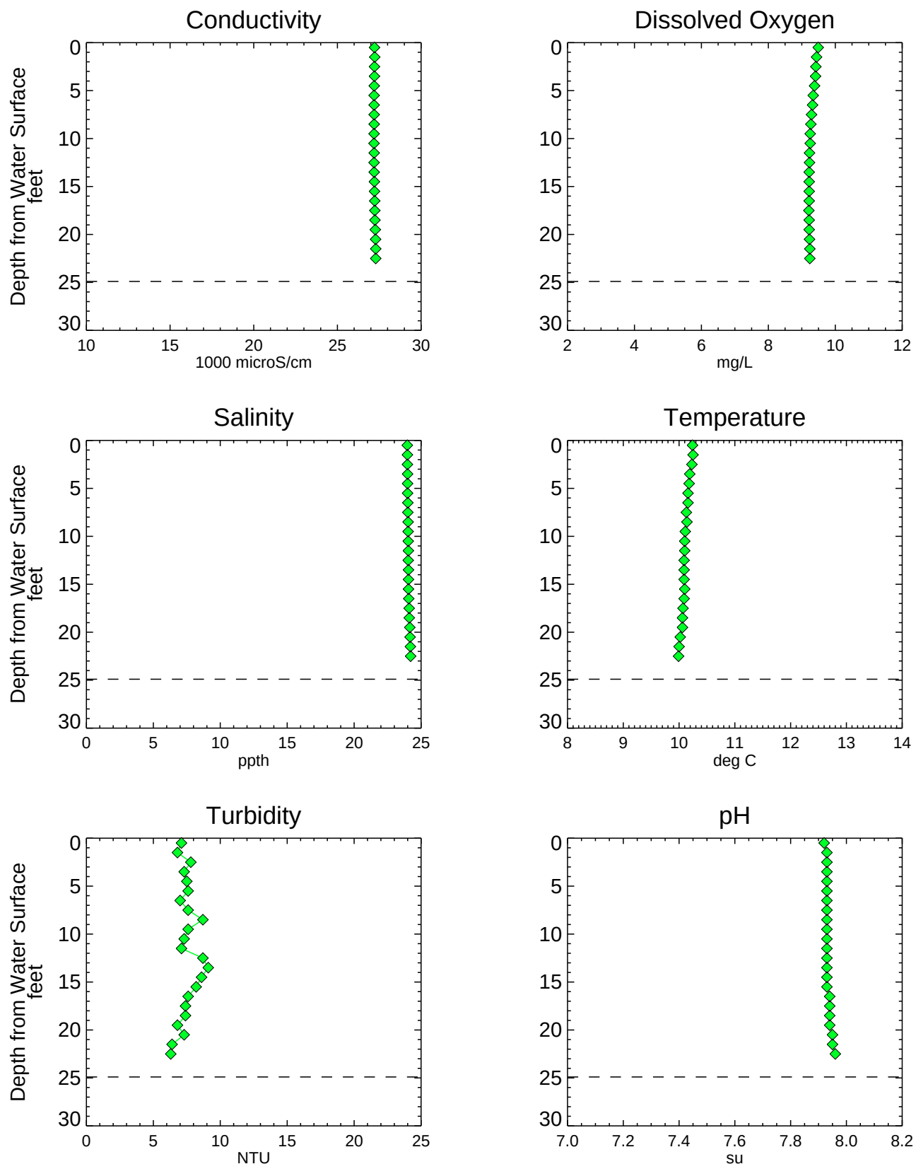
Figure A3-32 Analytical Water Quality Depth Profiles - NC020SW Phase 1 RI Data Summary Report - Submittal No. 1 Newtown Creek RI/FS
