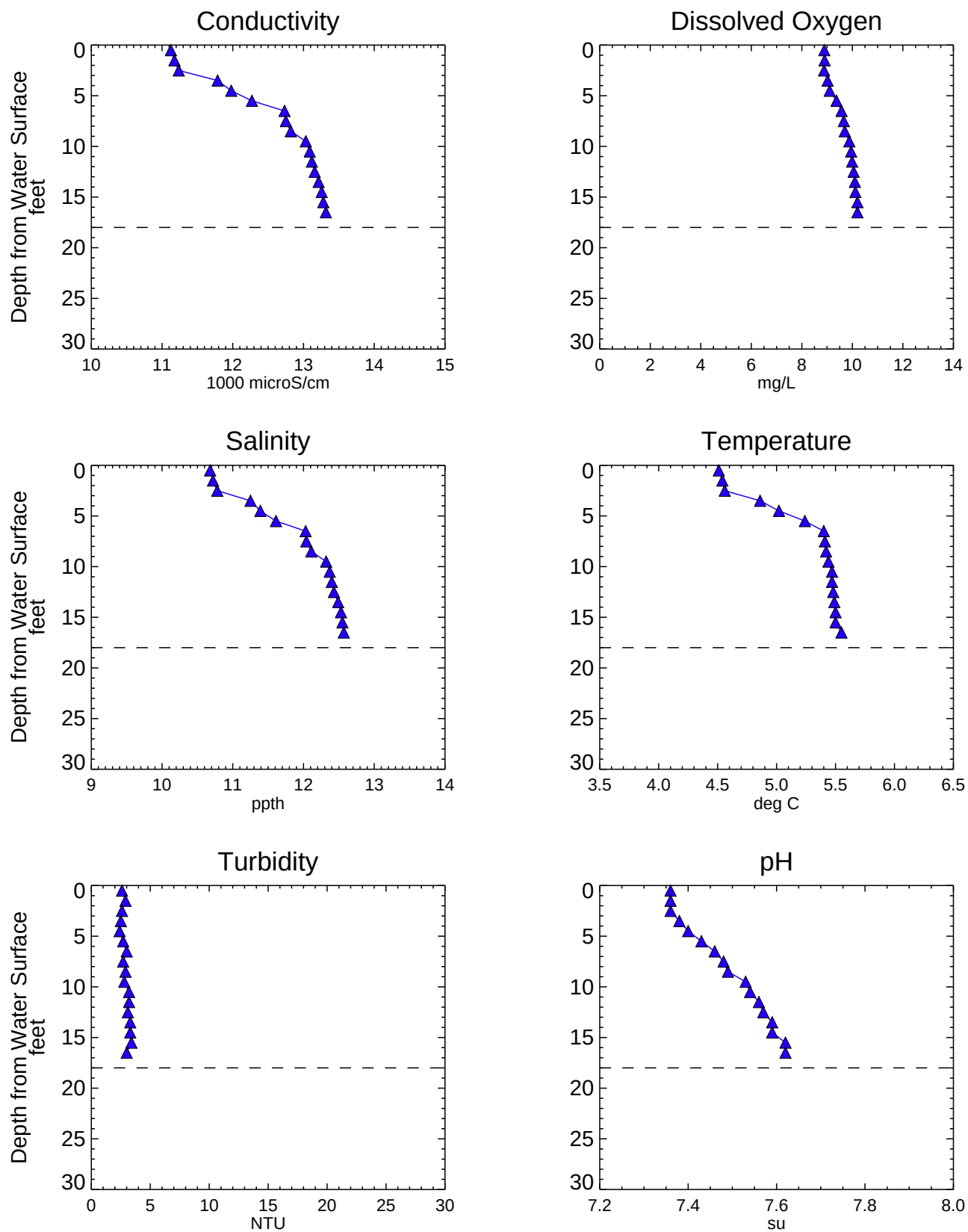
Figure A3-9 Analytical Water Quality Depth Profiles - NC070SW Phase 1 RI Data Summary Report - Submittal No. 1 Newtown Creek RI/FS
