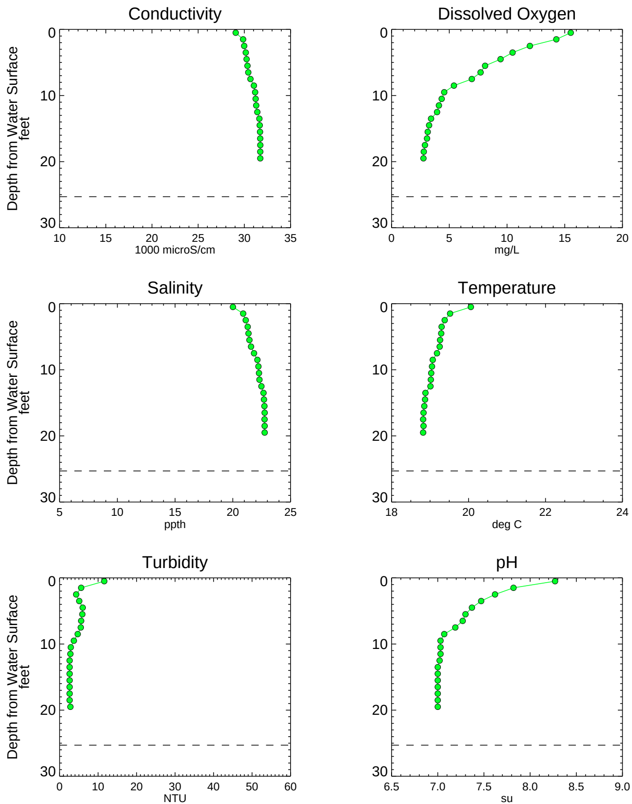
Figure A3-72 Analytical Water Quality Depth Profiles - NC079SW Phase 1 RI Data Summary Report - Submittal No. 1 Newtown Creek RI/FS
