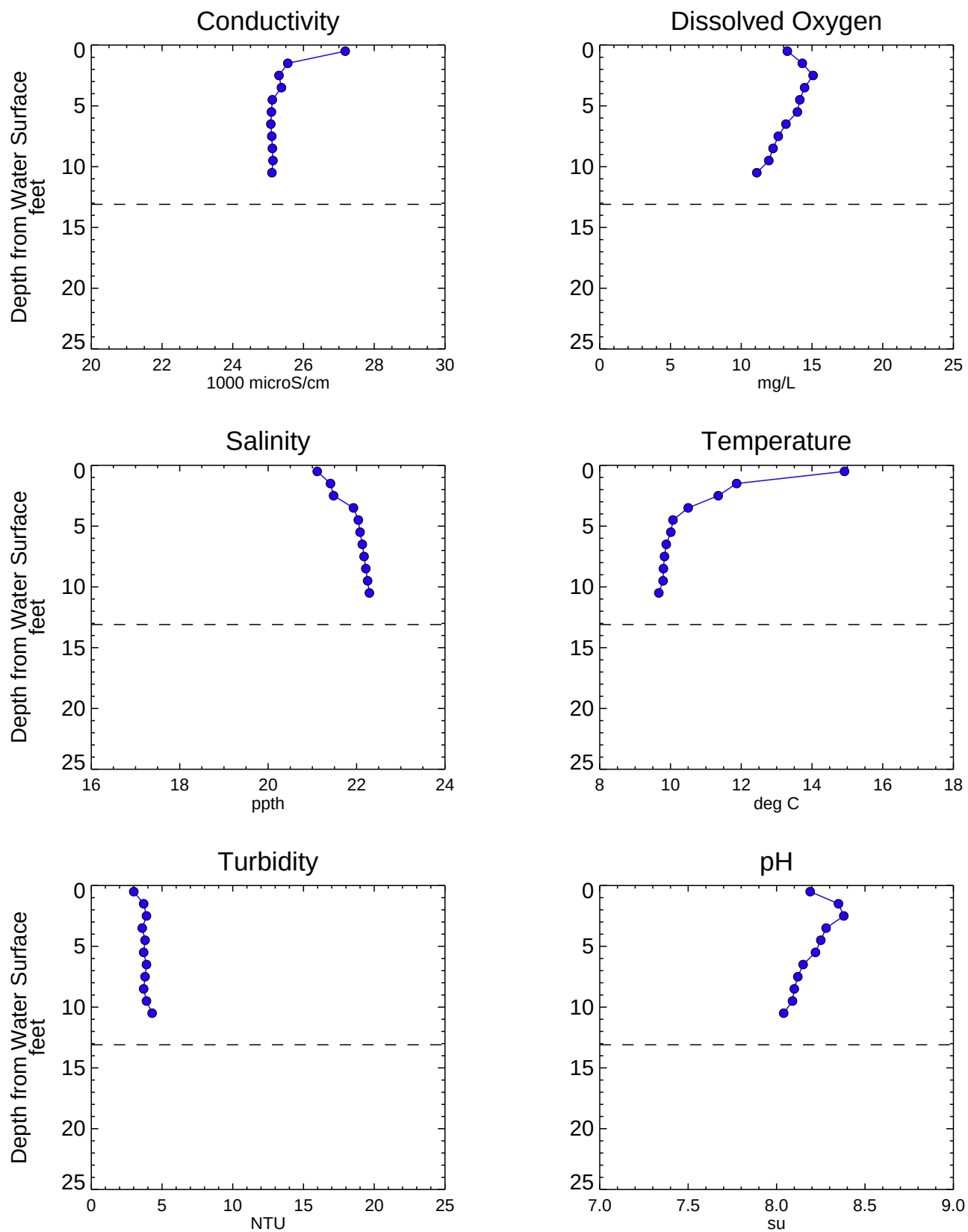
Figure A3-27 Analytical Water Quality Depth Profiles - EK006SW Phase 1 RI Data Summary Report - Submittal No. 1 Newtown Creek RI/FS
