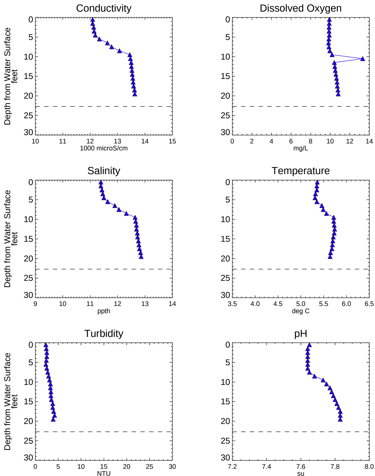
Figure A3-7 Analytical Water Quality Depth Profiles - NC046SW Phase 1 RI Data Summary Report - Submittal No. 1 Newtown Creek RI/FS
