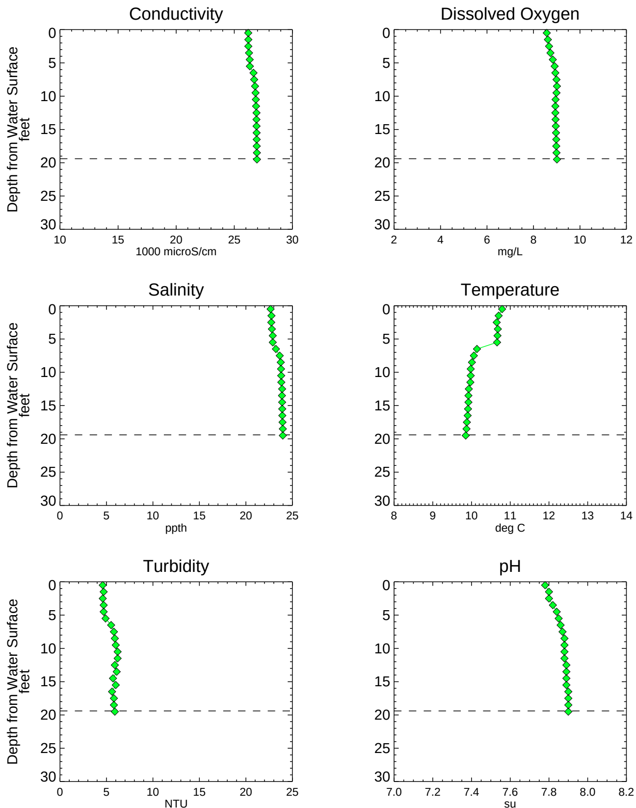
Figure A3-33 Analytical Water Quality Depth Profiles - DK001SW Phase 1 RI Data Summary Report - Submittal No. 1 Newtown Creek RI/FS
