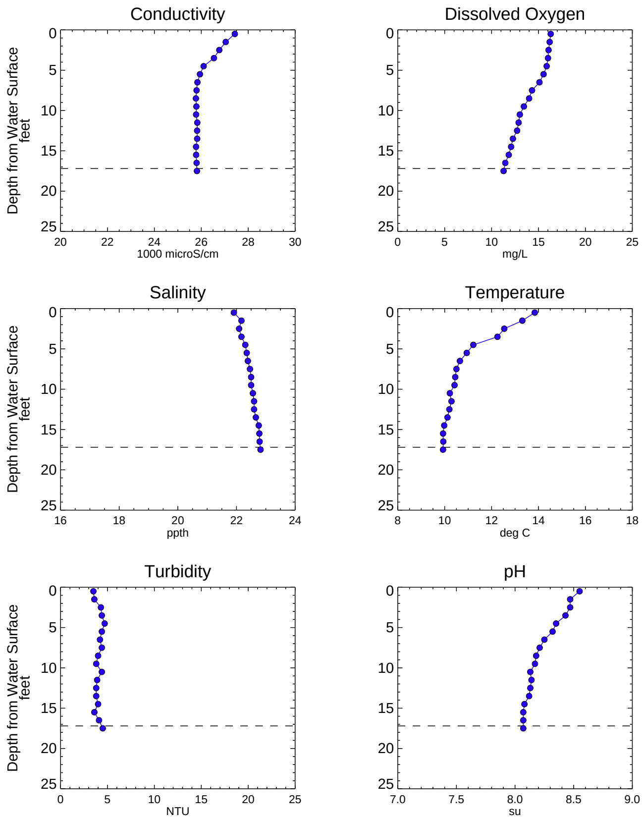
Figure A3-18 Analytical Water Quality Depth Profiles - DK001SW Phase 1 RI Data Summary Report - Submittal No. 1 Newtown Creek RI/FS
