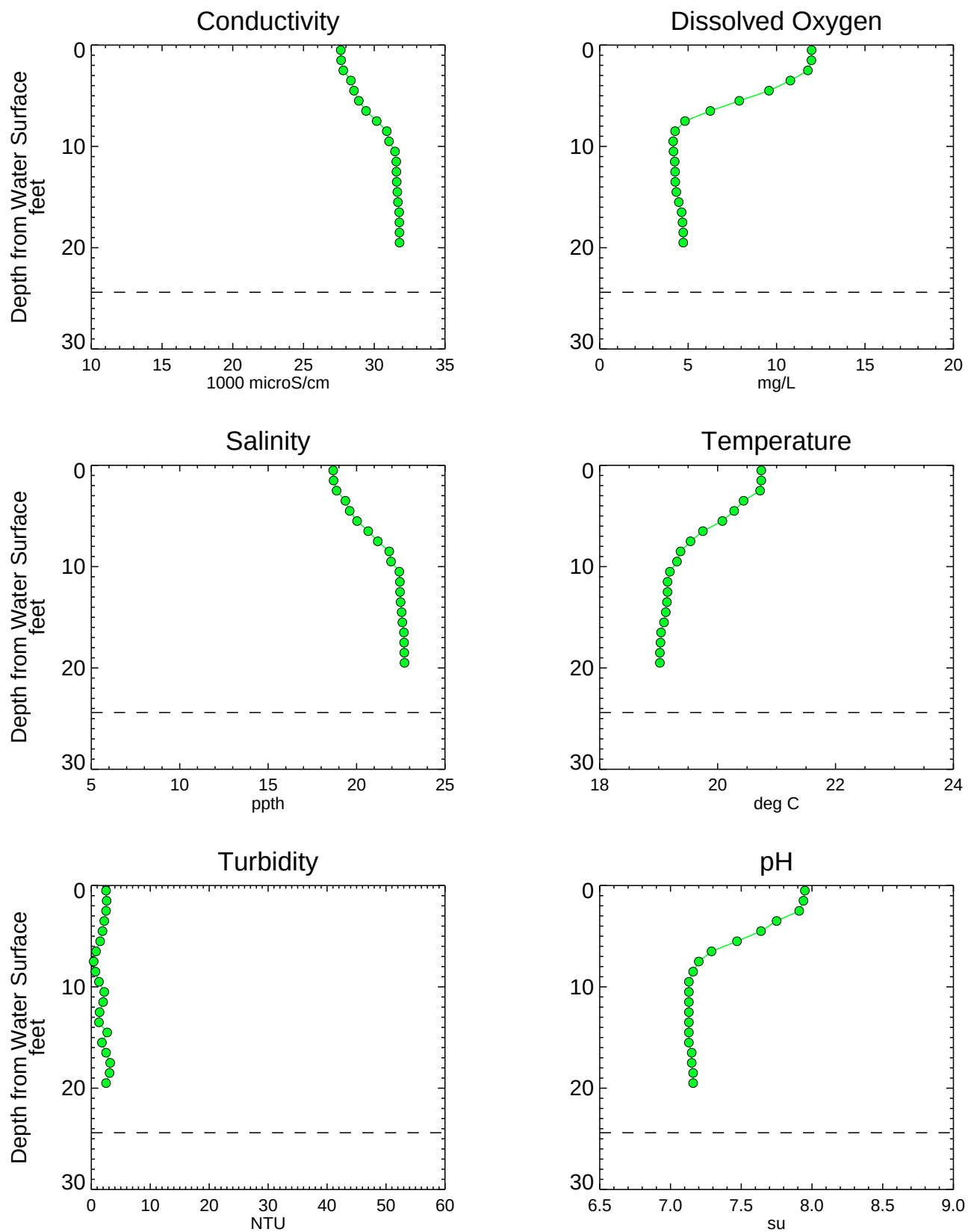
Figure A3-66 Analytical Water Quality Depth Profiles - NC034SW Phase 1 RI Data Summary Report - Submittal No. 1 Newtown Creek RI/FS
