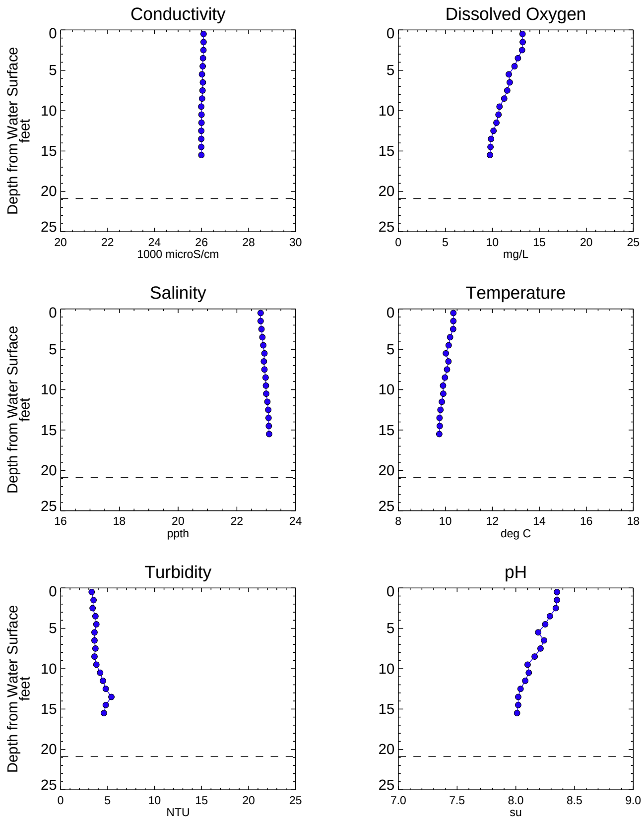
Figure A3-16 Analytical Water Quality Depth Profiles - NC007SW Phase 1 RI Data Summary Report - Submittal No. 1 Newtown Creek RI/FS
