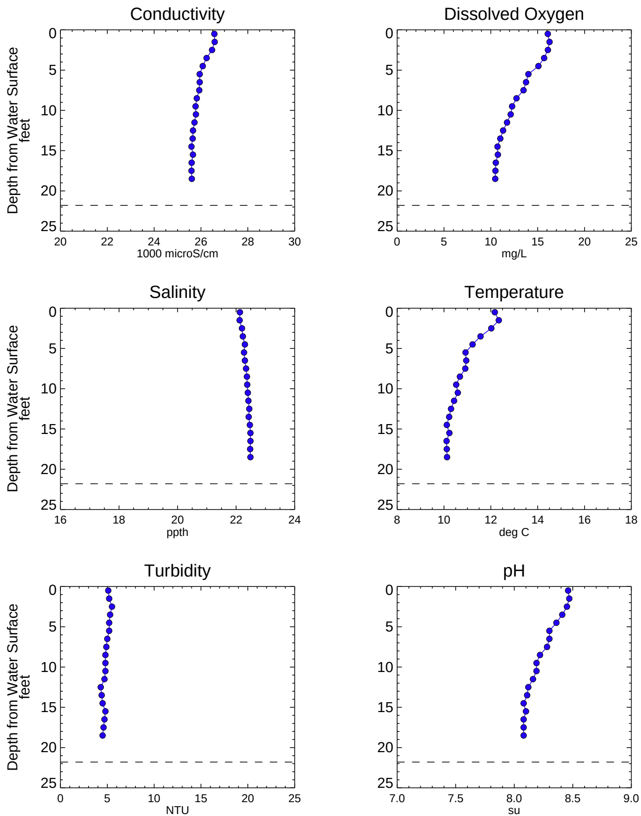
Figure A3-26 Analytical Water Quality Depth Profiles - NC079SW Phase 1 RI Data Summary Report - Submittal No. 1 Newtown Creek RI/FS
