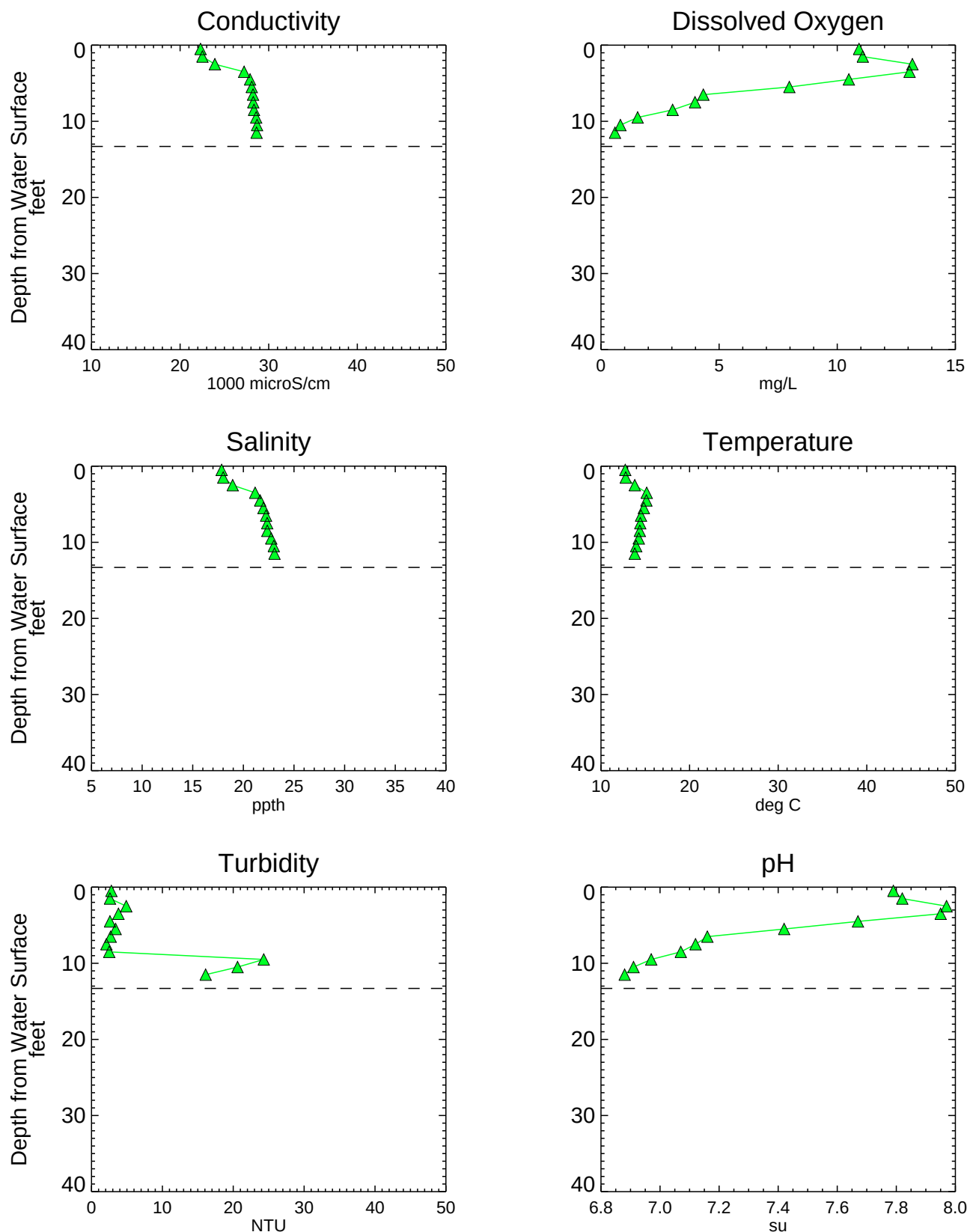
Figure A3-52 Analytical Water Quality Depth Profiles - DK011SW Phase 1 RI Data Summary Report - Submittal No. 1 Newtown Creek RI/FS
