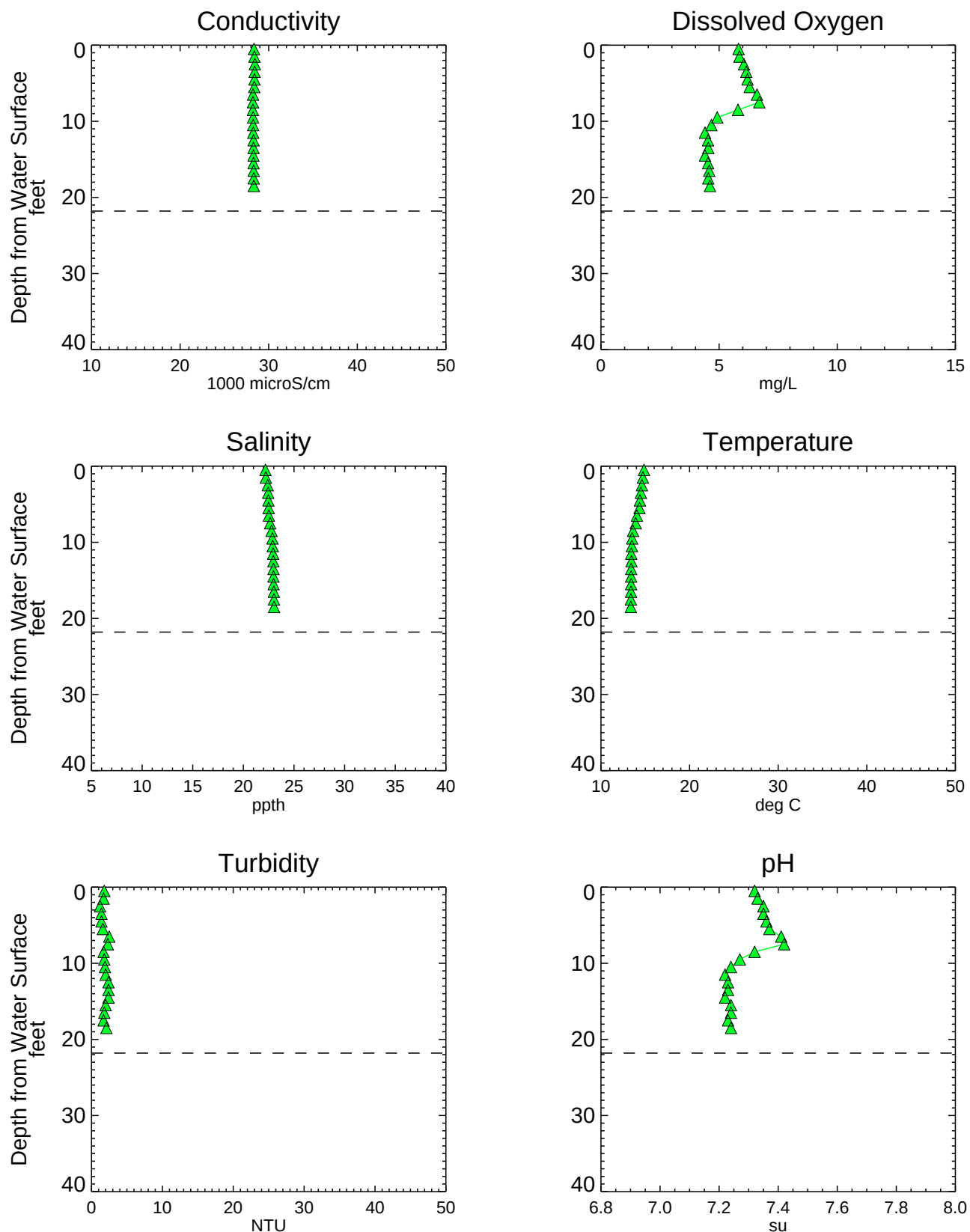
Figure A3-54 Analytical Water Quality Depth Profiles - NC068SW Phase 1 RI Data Summary Report - Submittal No. 1 Newtown Creek RI/FS
