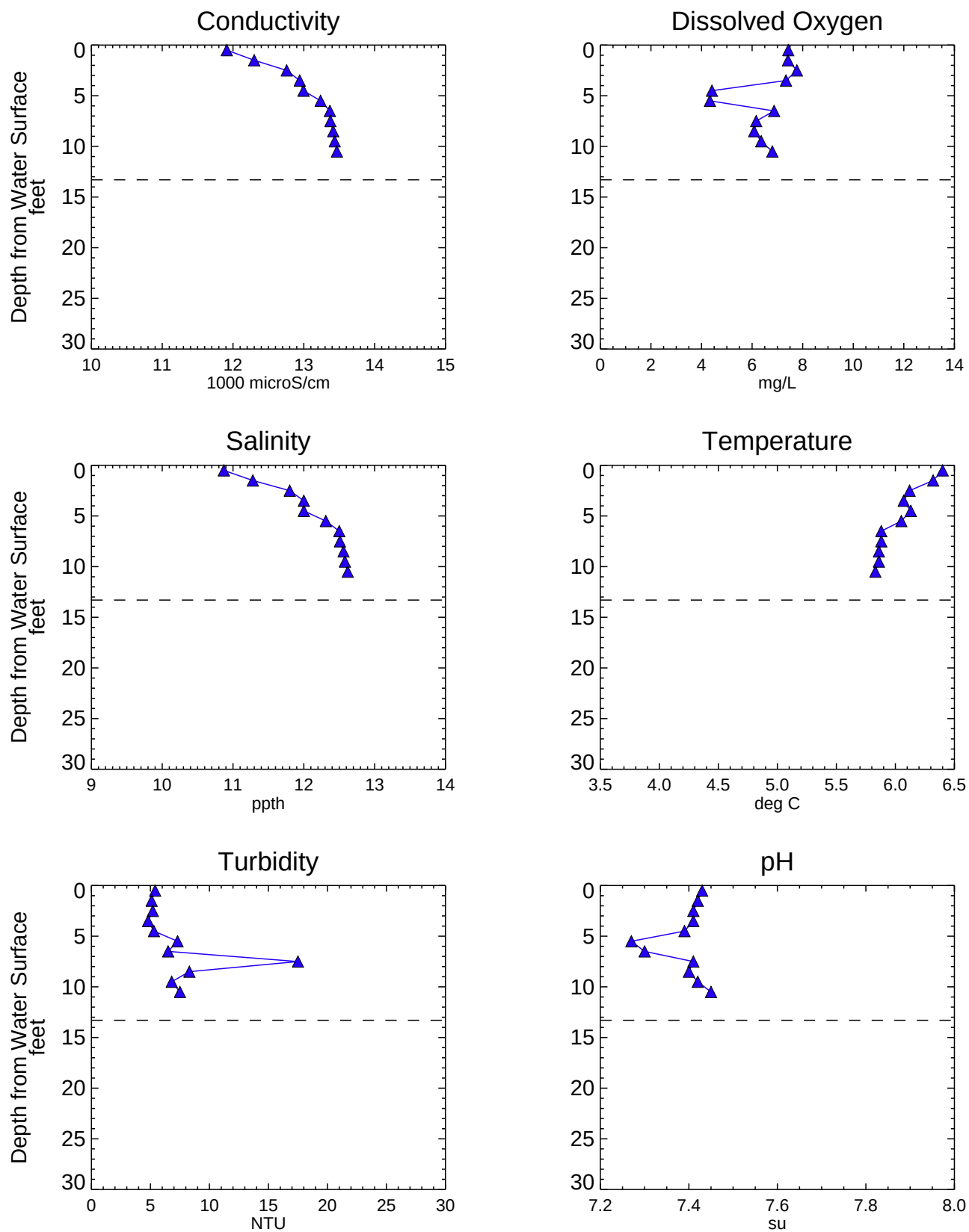
Figure A3-6 Analytical Water Quality Depth Profiles - DK011SW Phase 1 RI Data Summary Report - Submittal No. 1 Newtown Creek RI/FS
