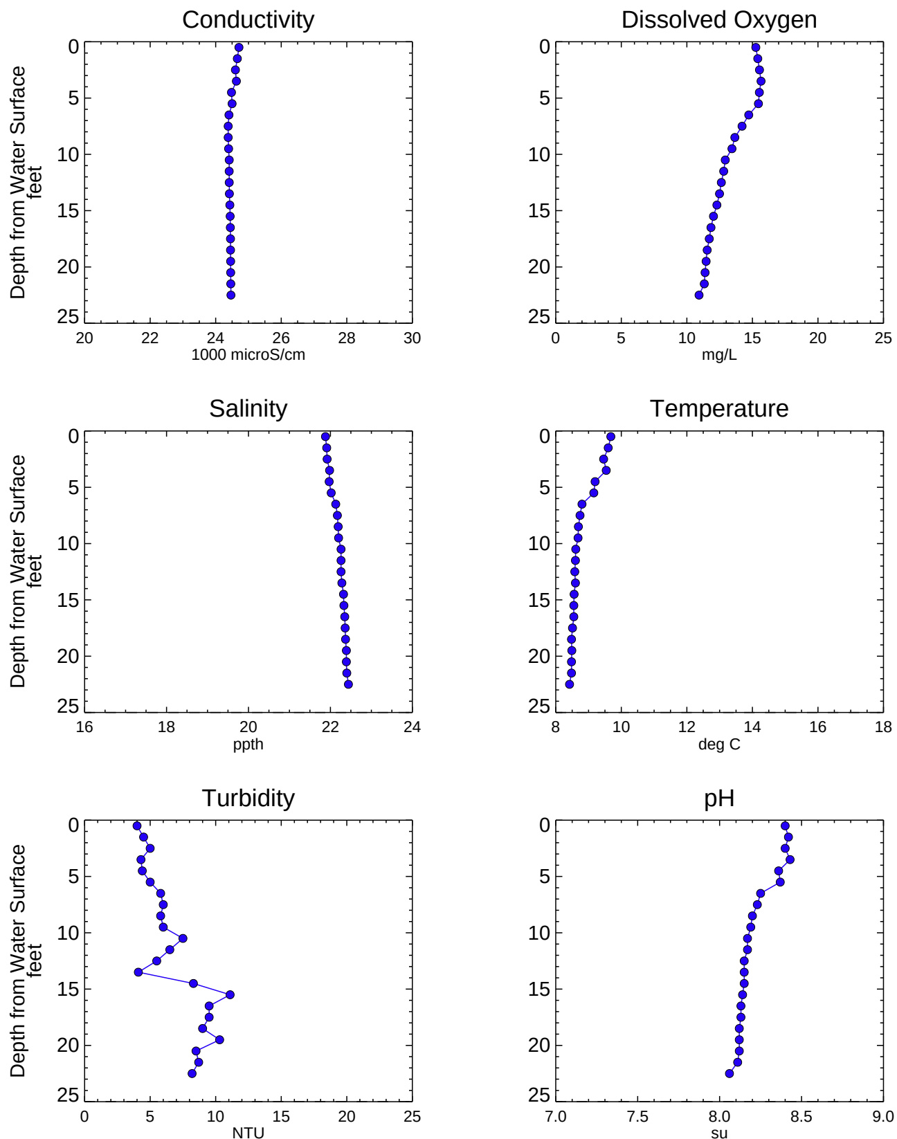
Figure A3-19 Analytical Water Quality Depth Profiles - WC001SW Phase 1 RI Data Summary Report - Submittal No. 1 Newtown Creek RI/FS
