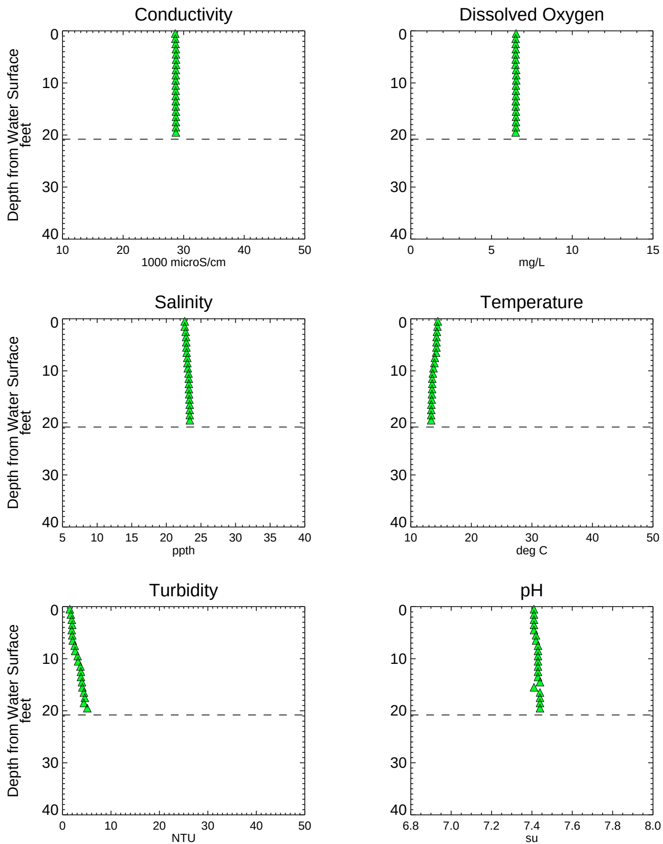
Figure A3-51 Analytical Water Quality Depth Profiles - NC034SW Phase 1 RI Data Summary Report - Submittal No. 1 Newtown Creek RI/FS
