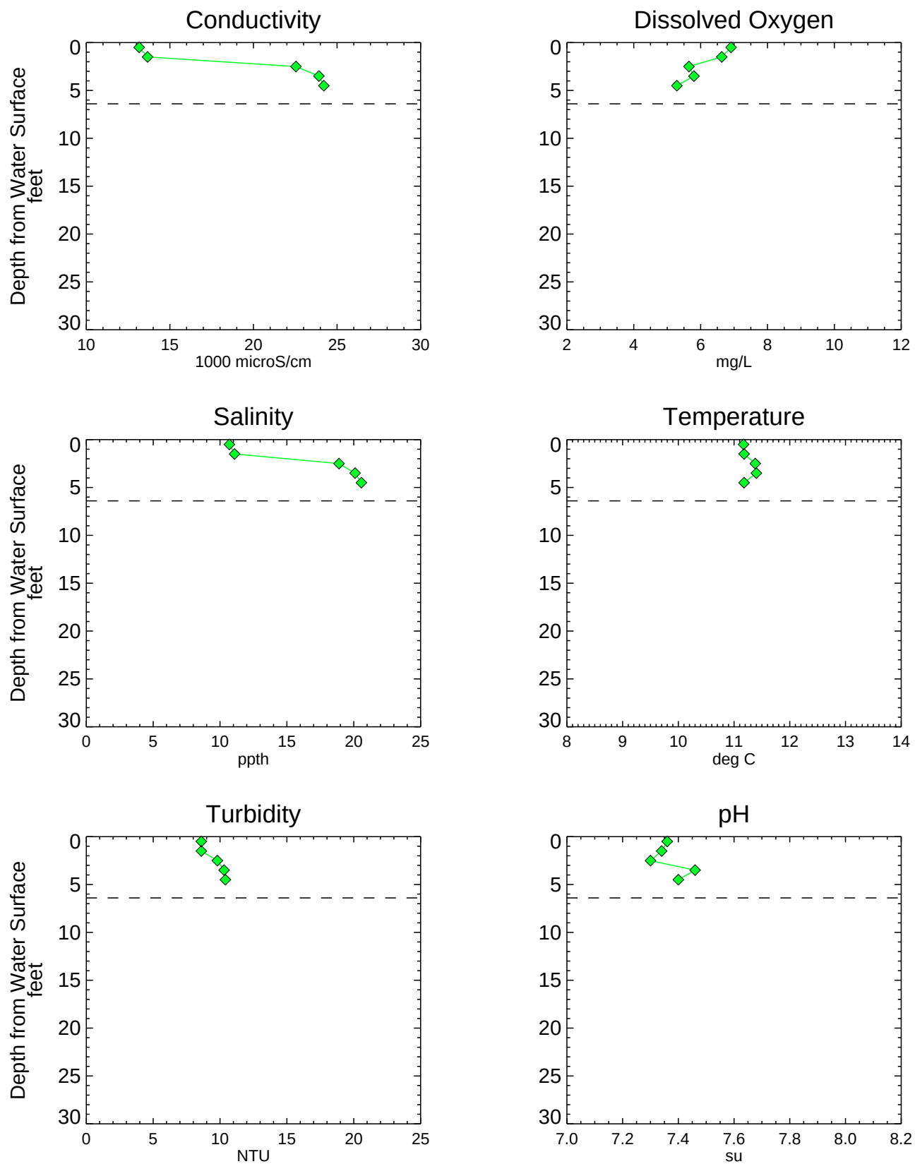
Figure A3-46 Analytical Water Quality Depth Profiles - EK022SW Phase 1 RI Data Summary Report - Submittal No. 1 Newtown Creek RI/FS
