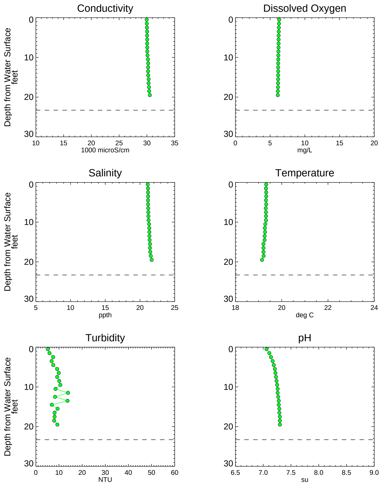
Figure A3-62 Analytical Water Quality Depth Profiles - NC007SW Phase 1 RI Data Summary Report - Submittal No. 1 Newtown Creek RI/FS
