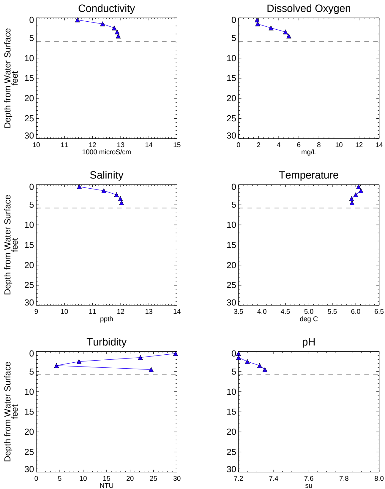
Figure A3-13 Analytical Water Quality Depth Profiles - EB010SW Phase 1 RI Data Summary Report - Submittal No. 1 Newtown Creek RI/FS
