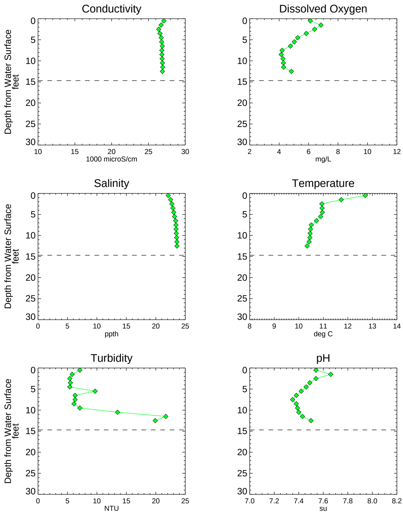
Figure A3-37 Analytical Water Quality Depth Profiles - DK011SW Phase 1 RI Data Summary Report - Submittal No. 1 Newtown Creek RI/FS
