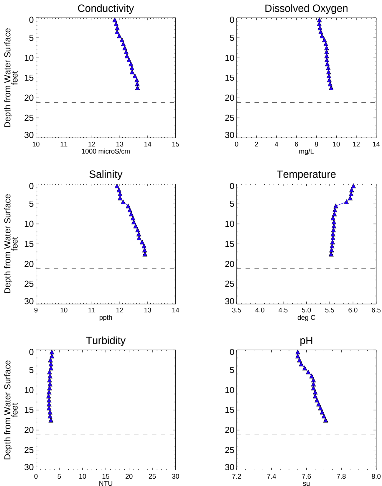
Figure A3-11 Analytical Water Quality Depth Profiles - NC079SW Phase 1 RI Data Summary Report - Submittal No. 1 Newtown Creek RI/FS
