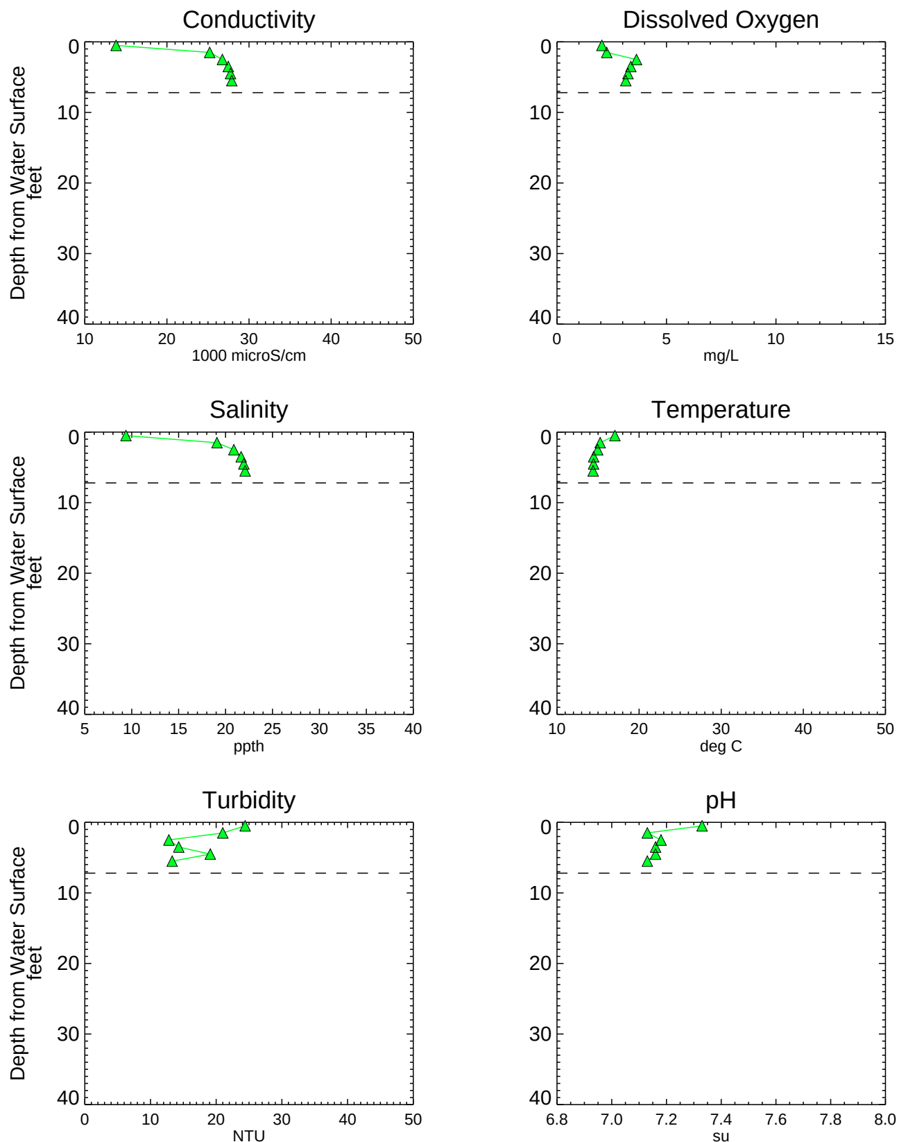
Figure A3-61 Analytical Water Quality Depth Profiles - EK022SW Phase 1 RI Data Summary Report - Submittal No. 1 Newtown Creek RI/FS
