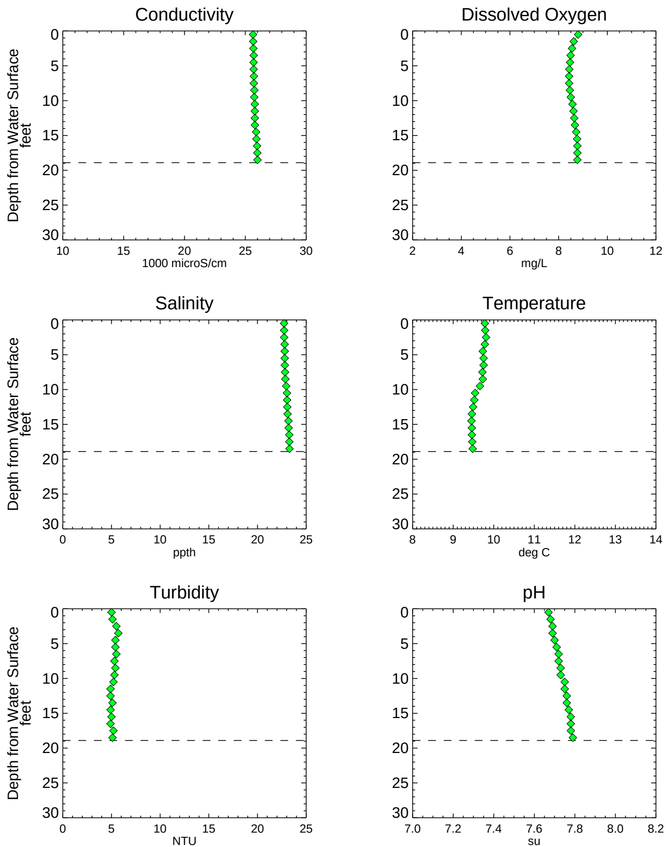
Figure A3-31 Analytical Water Quality Depth Profiles - NC007SW Phase 1 RI Data Summary Report - Submittal No. 1 Newtown Creek RI/FS
