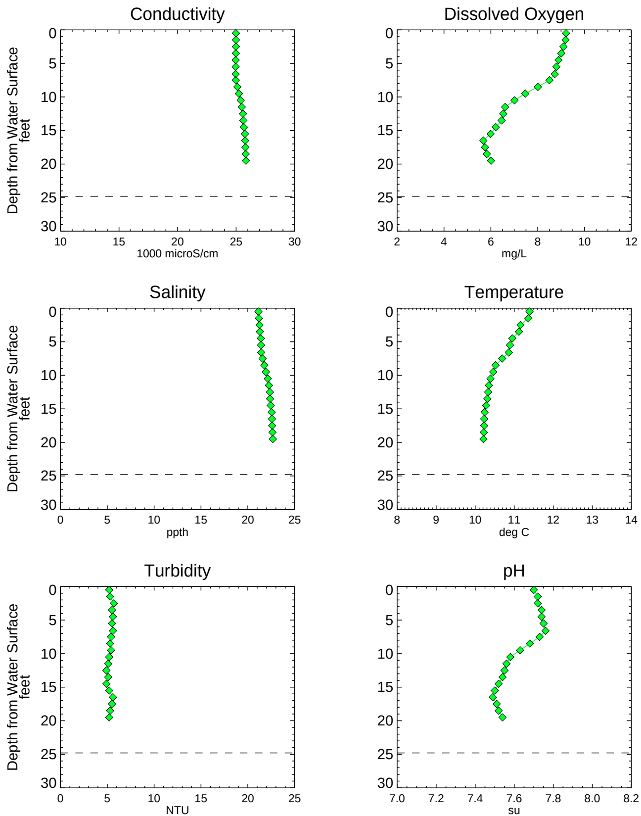
Figure A3-39 Analytical Water Quality Depth Profiles - NC068SW Phase 1 RI Data Summary Report - Submittal No. 1 Newtown Creek RI/FS
