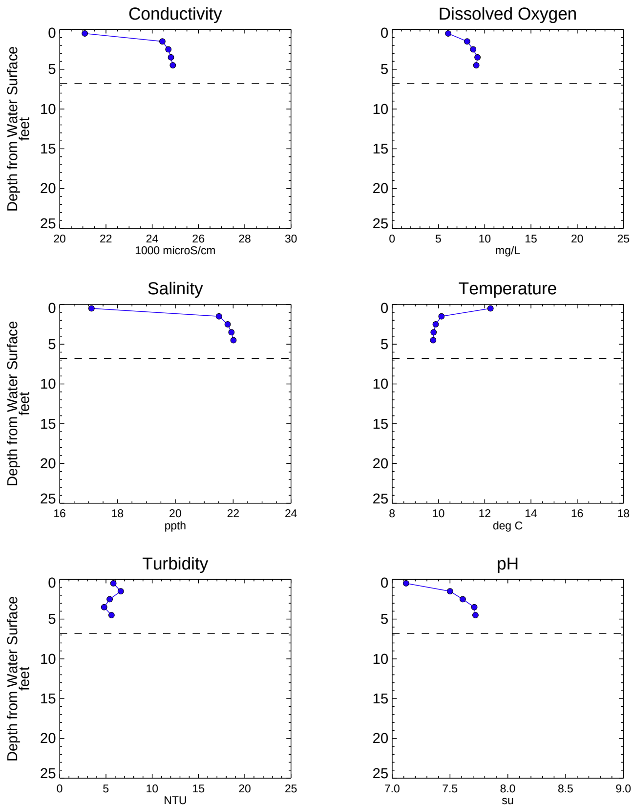
Figure A3-30 Analytical Water Quality Depth Profiles - EK022SW Phase 1 RI Data Summary Report - Submittal No. 1 Newtown Creek RI/FS
