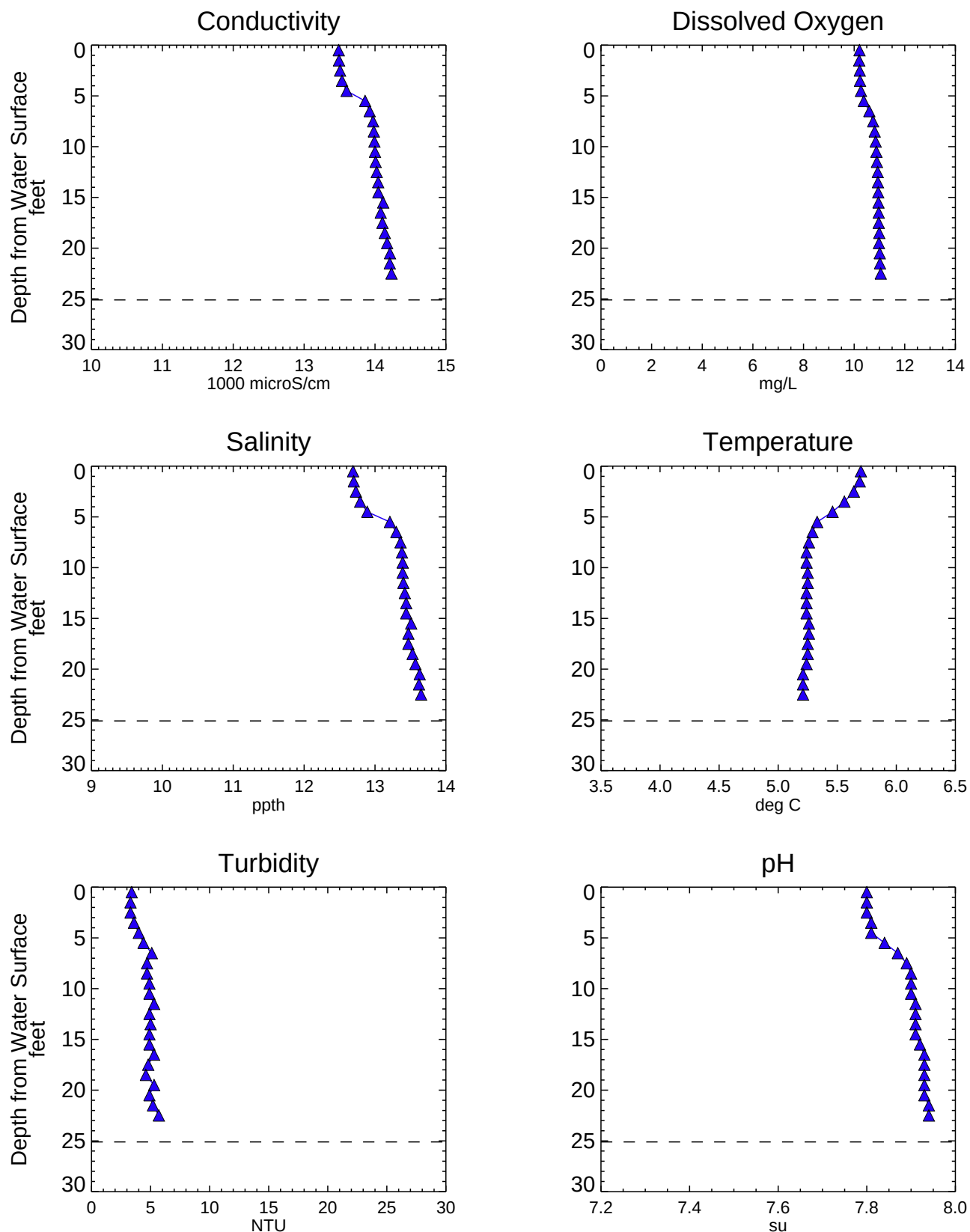
Figure A3-4 Analytical Water Quality Depth Profiles - WC001SW Phase 1 RI Data Summary Report - Submittal No. 1 Newtown Creek RI/FS
