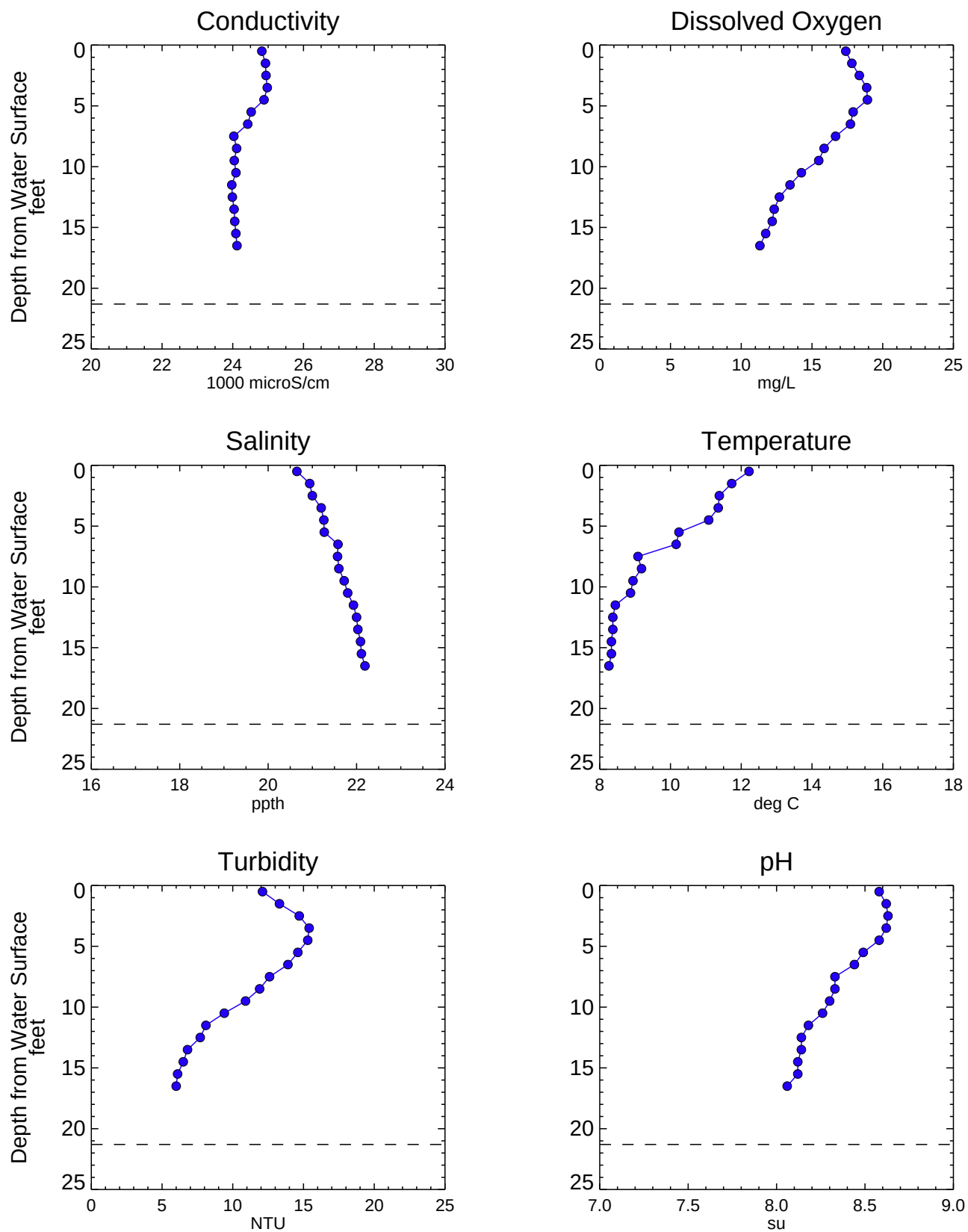
Figure A3-23 Analytical Water Quality Depth Profiles - NC068SW Phase 1 RI Data Summary Report - Submittal No. 1 Newtown Creek RI/FS
