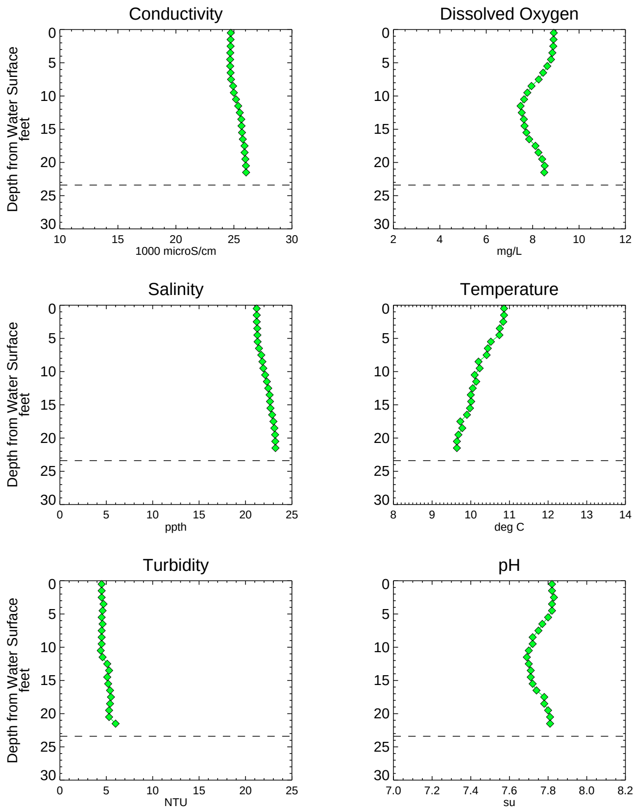
Figure A3-36 Analytical Water Quality Depth Profiles - NC034SW Phase 1 RI Data Summary Report - Submittal No. 1 Newtown Creek RI/FS
