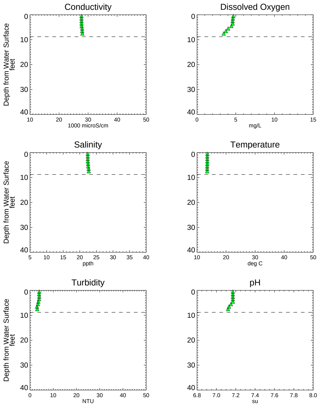
Figure A3-60 Analytical Water Quality Depth Profiles - EK014SW Phase 1 RI Data Summary Report - Submittal No. 1 Newtown Creek RI/FS
