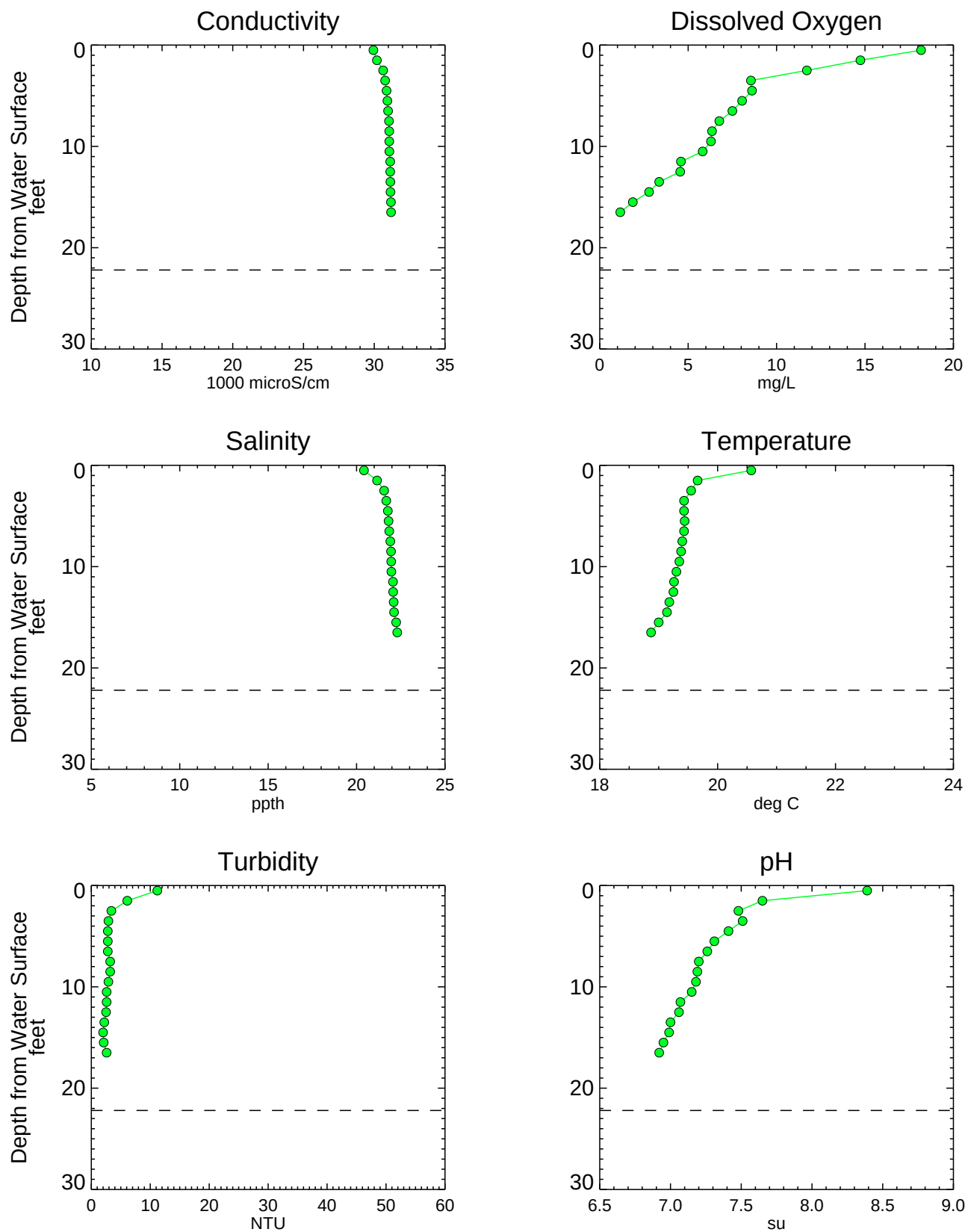
Figure A3-73 Analytical Water Quality Depth Profiles - EK006SW Phase 1 RI Data Summary Report - Submittal No. 1 Newtown Creek RI/FS
